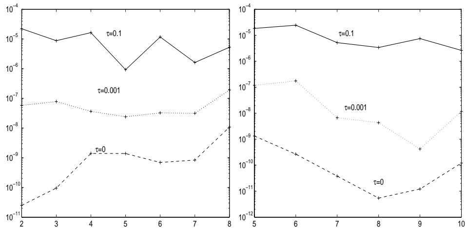
Fig. 2: relative errors; eigenvalues in (0,0.2) and (0.2,0.5)
