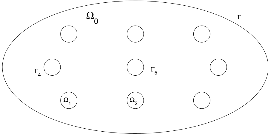
Fig. 1: Domain \Omega_0
