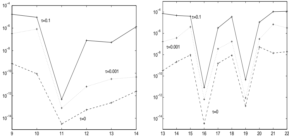
Fig. 3: relative errors; eigenvalues in (0.5, 1.0) and (1.0, 2.0)
