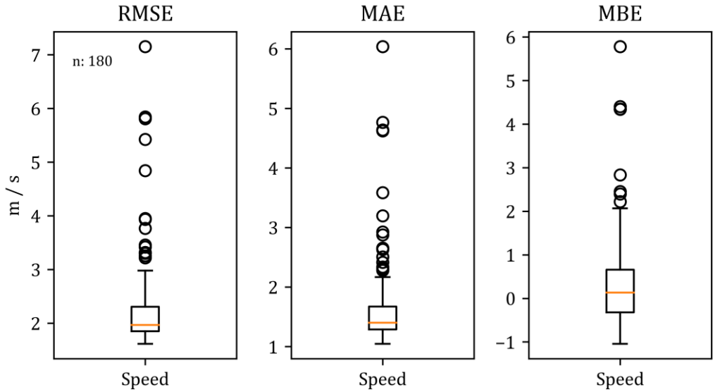
Figure 7: Overall statistical results for wind speed. Speed differences were accounted and are given in m/s. Size of dataset was n = 180.
