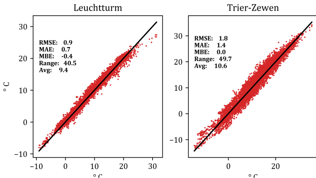
Figure 6: Best fits of COSMO data and observation data. The best in RMSE and MAE is Leuchtturm and in |MBE| Trier-Zewen.
