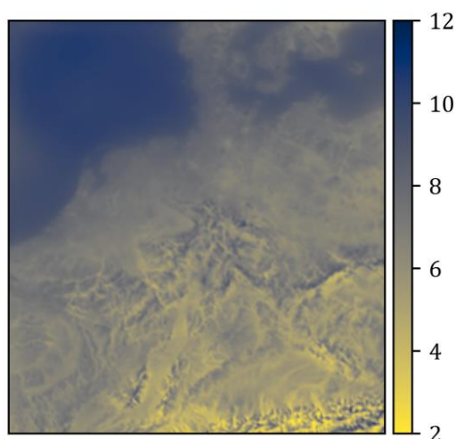
Figure 14: Mean wind speed at 122.32 m distribution 2009 in the data set in m/s. Every pixel represents a \sim 2.8 \times 2.8 km grid cell.
