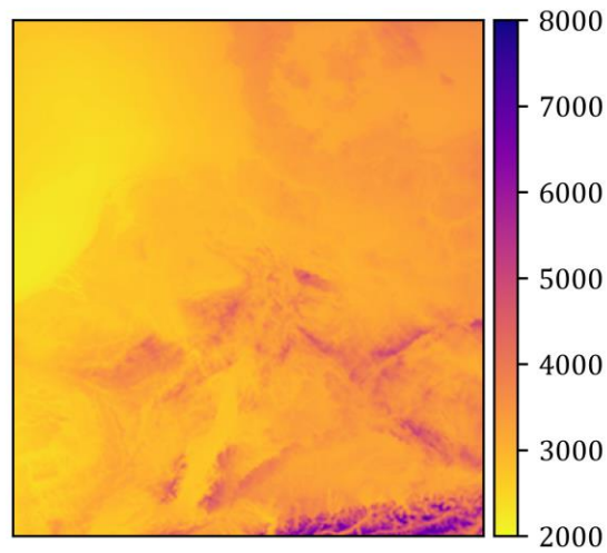
Figure 13: GTZ distribution 2009 in the data set in K. Every pixel represents a ~2.8x2.8 km grid cell.
