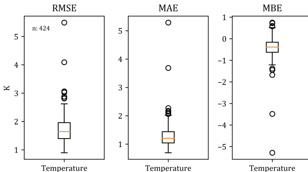
Figure 4: Overall statistical results for temperature. Temperature differences were accounted and are given in Kelvin. Size of dataset was n = 424.
