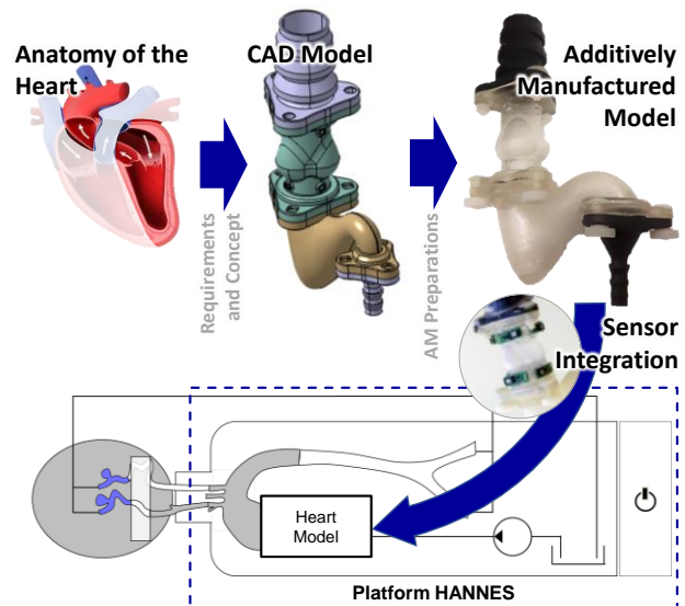
Figure 1: Development of a heart model for the medical simulator HANNES for evaluating the performance of aortic valve implants after TAVI procedure (partly based on [3],[8])
