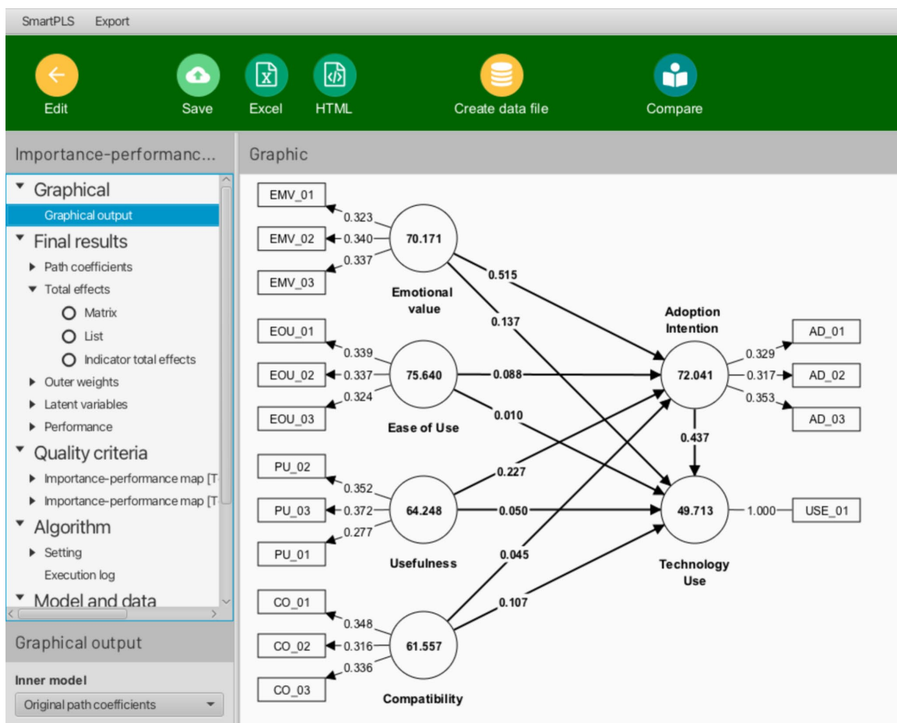
Fig. 8 IPMA results
