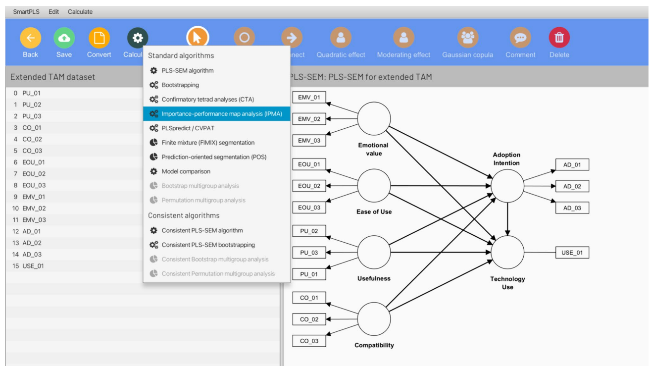
Fig. 6 Modeling window
