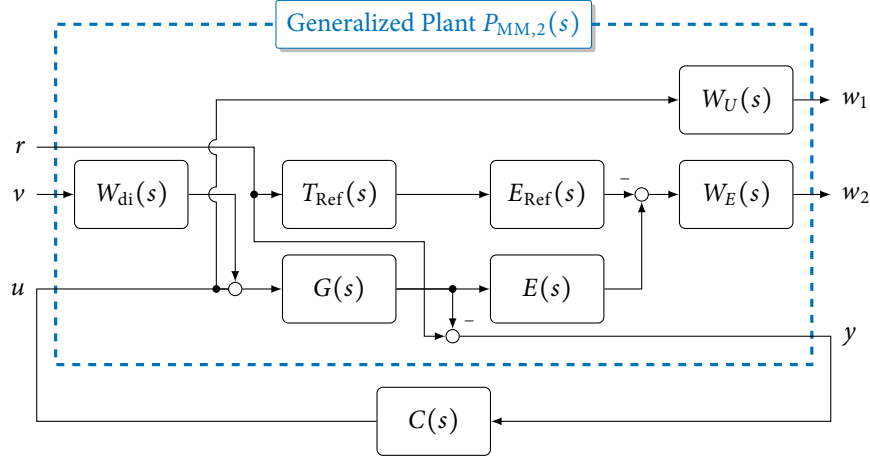
Figure 6.6: Generalized plant for the second model matching design.
