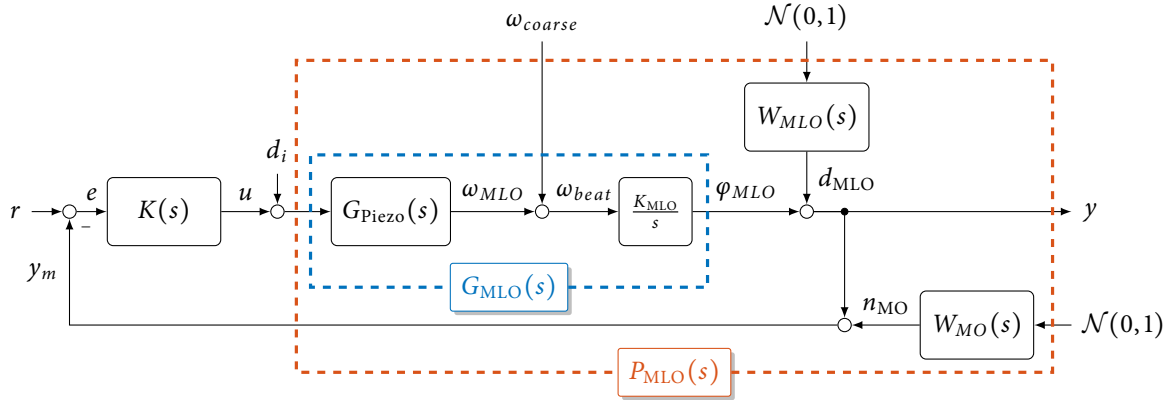
Figure 4.22: Control loop for the MLO system with additional coloring filter.
