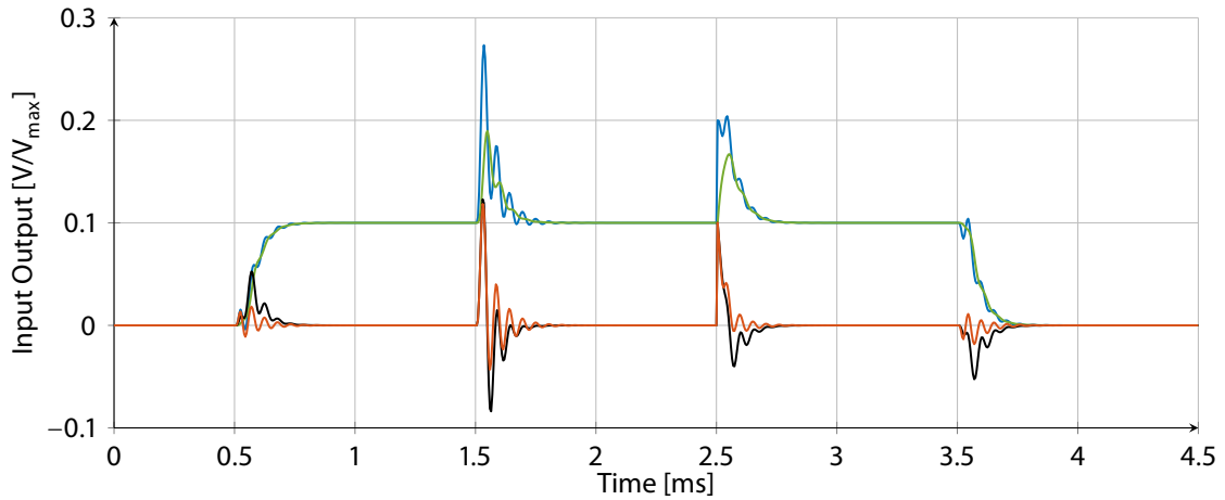
Figure 6.7: Simulation of the error after the BAM (—) and the L2RF (—) end-station with the difference (—) for the second design, compare to the previous difference (—).
