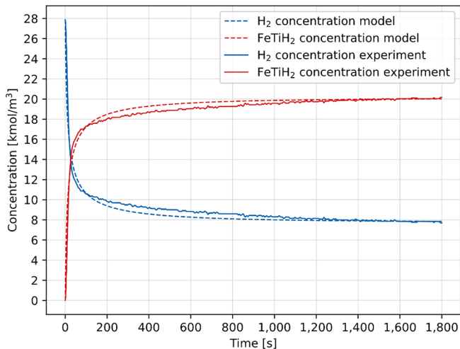
Fig. 5. Comparison of developed reaction kinetics and experimental data from [18] for hydrogen absorption.
