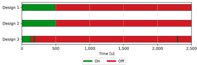
Fig. 16. Heating settings for design concept 1, design concept 2 and design concept 3 with RHC.
