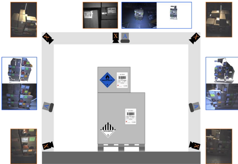
Figure 33: Shipment handling camera setup
