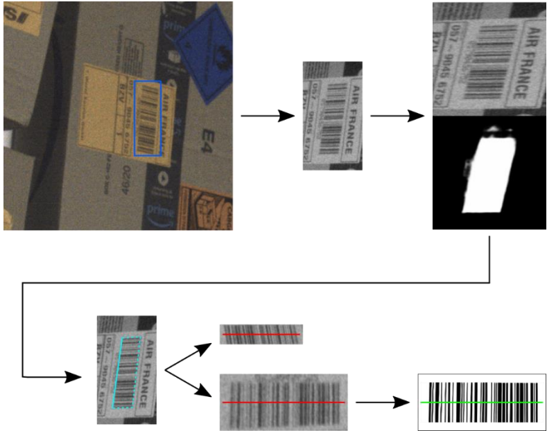
Figure 36: Main steps of the barcode detection and decoding pipeline
