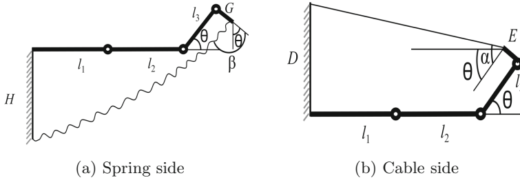
Fig. 3. Simplified kinematic model of the robot
