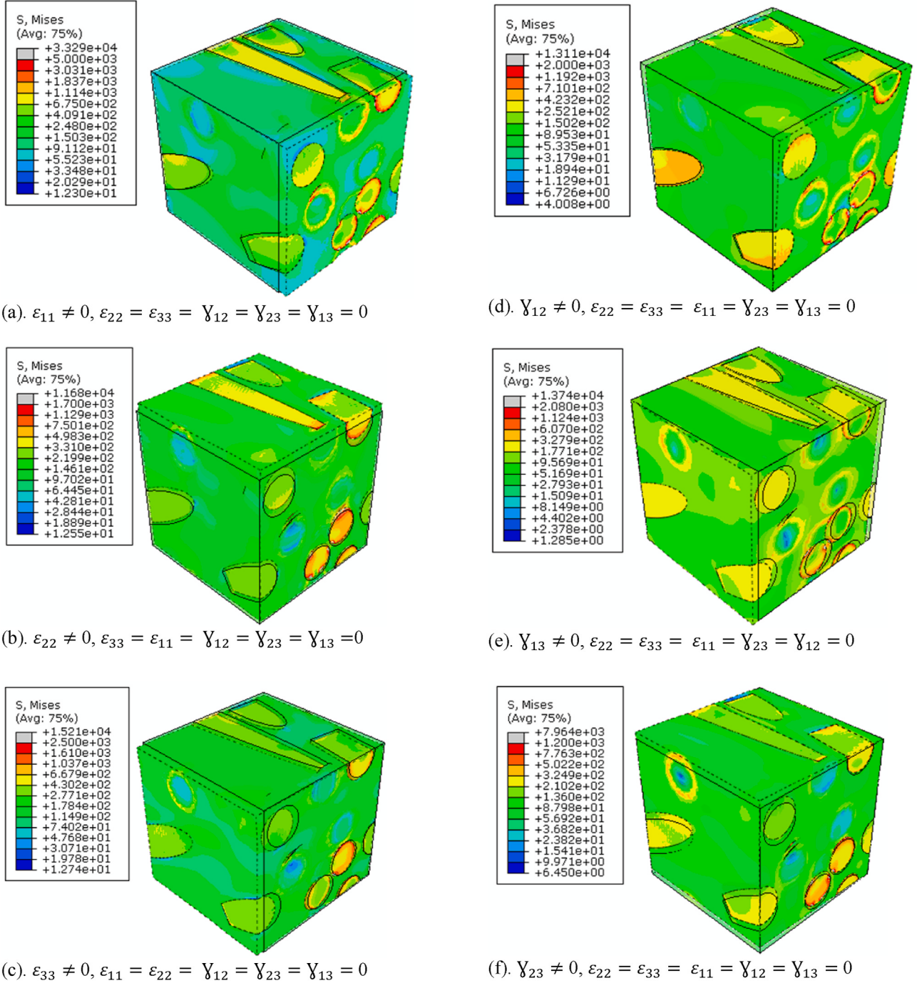
Fig. 12. The stress distributions within the micro-scale model of the RVE of a 3D printed composite part, composed of Short Glass Fiber (SGF) reinforced Polyamide (PA), are analysed under six states of uniaxial and shear strains. The deformed and undeformed shapes of the micro-scale RVE are represented by dashed and solid lines, respectively. It must be noted that the units in this Figure for all RVEs are in Pa.
