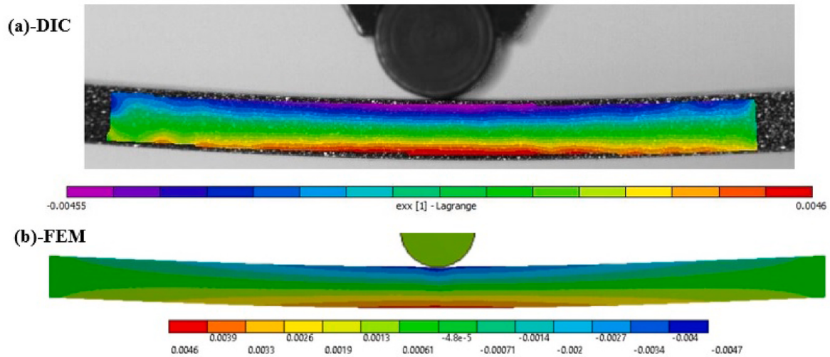
Fig. 15. (a) DIC and (b) FE computed strain distribution maps of SCF/PA 3D printed specimens with 0^\circ raster at the maximum deflection of 1.5 mm with the corresponding load of 92 N.
