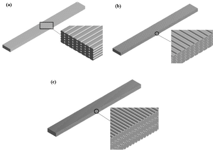
Fig. 14. Schematic representation of SCF/PA 3D printed Three-Point Bending specimens with different raster angle and build orientation. (a) raster angle of 0^\circ , (b) raster angle of 90^\circ , (c) build orientation of upright.
