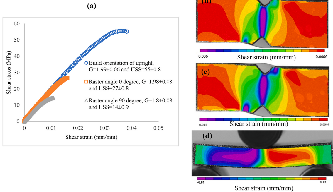
Fig. 10. (a) Shear stress-strain curves for different build orientation and raster angle of 3D FFF-printed 30% SGF/PA measured by DIC system. DIC strain distribution maps in terms of in-plane and inter-laminar shear strains prior to the fracture point for 3D FFF-printed tensile specimens of (b) Iosipescu shear test sample with the build orientation of upright as shown in Fig. 2d–(c) Iosipescu shear test sample with 0° raster angle as shown in Fig. 2f. (d) SBS test sample with 90° raster angle as shown in Fig. 2e. (At least five specimens of each condition were tested and the confidence level for all intervals is 95%).
