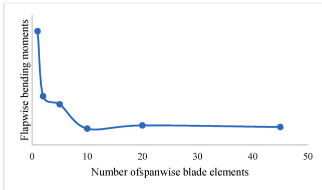
Fig. 5. Grid sensitivity analysis to determine the number of spanwise blade element at the reference seawater velocity of 2 m/s.
