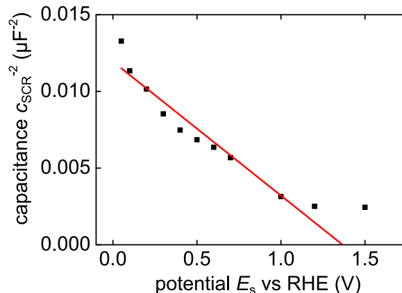
Fig. 3. Mott-Schottky plot of a bulk silicon electrode in 1 \text{ mol l}^{-1} perchloric acid. The capacitance determined by EIS is plotted as c_{\text{SCR}}^{-2} versus the respective static potential E_s . c_{\text{SCR}} is determined via EIS measurements with frequencies in the range of 1 MHz to 500 MHz and static potentials in the range of 0.05 – 1.5 V. A linear fit to the Mott-Schottky plot yields a flatband potential of E_{\text{fb}} = 1.4 \pm 0.1 \text{ V} and a carrier concentration of N_a = (2.6 \pm 0.3) \cdot 10^{19} \text{ cm}^{-3} . The linear fit is only performed up until a potential of 1.0 V. The line of the fit is then prolonged to mark the flatband potential at c_{\text{SCR}}^{-2} = 0 .
