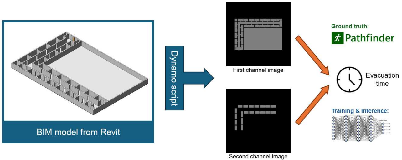
Figure 1: Our methodology, including the BIM model generation based on the parameters in Table 2, its image export via Dynamo, and the resulting tensor map with two channels. The first image channel encompasses walkable areas visualized in gray, the non-walkable areas in black, and the destination in white. The second channel resembles per-room densities at initialization.
