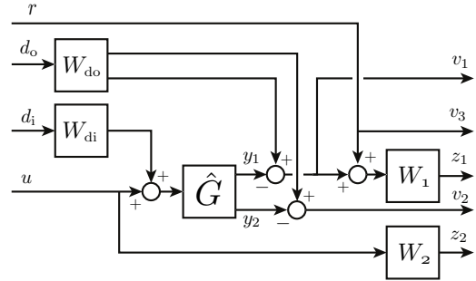
Fig. 3. General mixed sensitivity design for both swing-up and stabilizing LPV controller synthesis.
