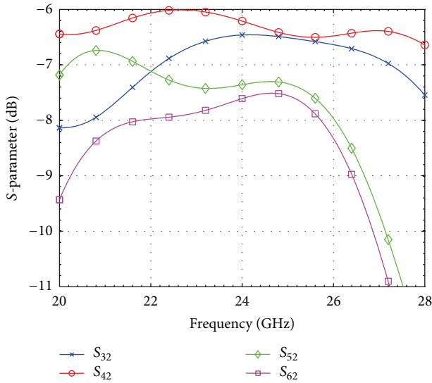
FIGURE 10: Six-port: simulated transmission from port 2 to the output ports.
