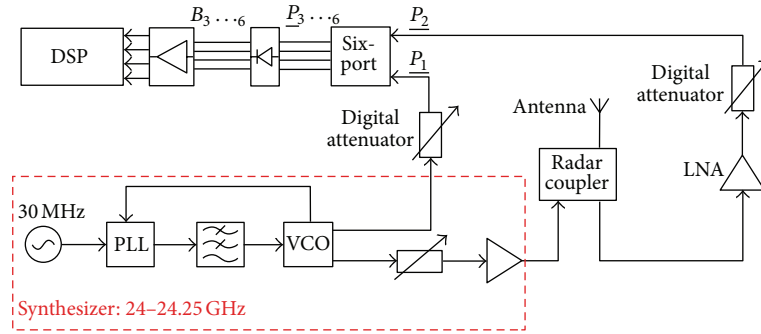
FIGURE 2: Schematic view of the radar front-end.
