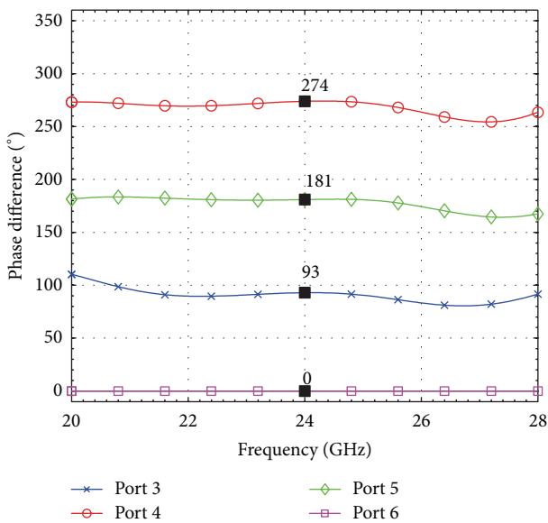
FIGURE 11: Simulated normalized phase difference at the output ports of the Six-port network (reference port 6 is set to 0°).
