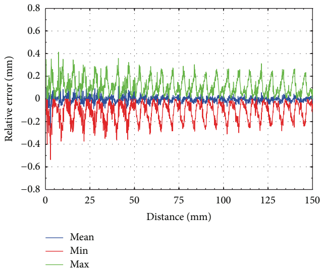
FIGURE 19: Relative measurement error.
