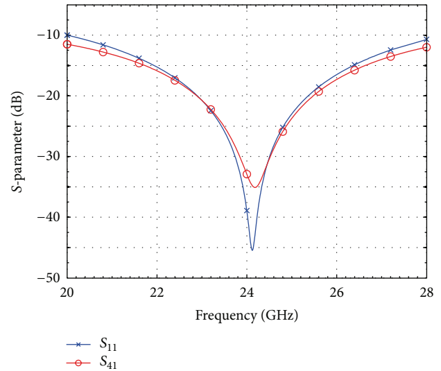
FIGURE 5: Simulated S_{11} and S_{41} of the quadrature hybrid coupler.
