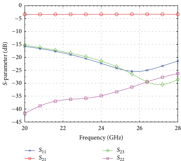
FIGURE 8: Simulated scattering parameters of power divider.
