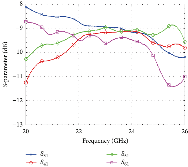
FIGURE 16: Six-port: measured transmission from port 1 to the output ports.
