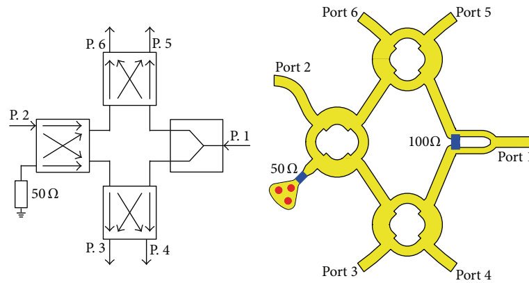
FIGURE 3: Schematic view and layout of the Six-port network.
