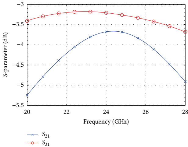
FIGURE 7: Simulated transmission coefficient of coupler.
