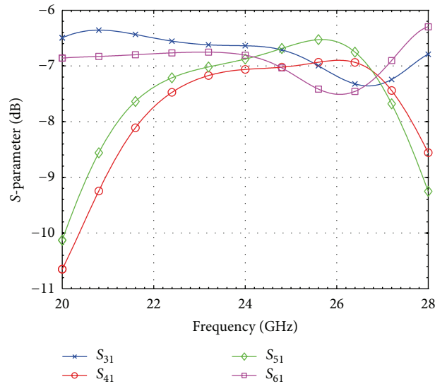
FIGURE 9: Six-port: simulated transmission from port 1 to the output ports.
