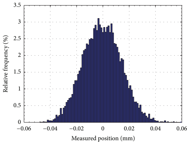
FIGURE 20: Standard deviation of measurement results.
