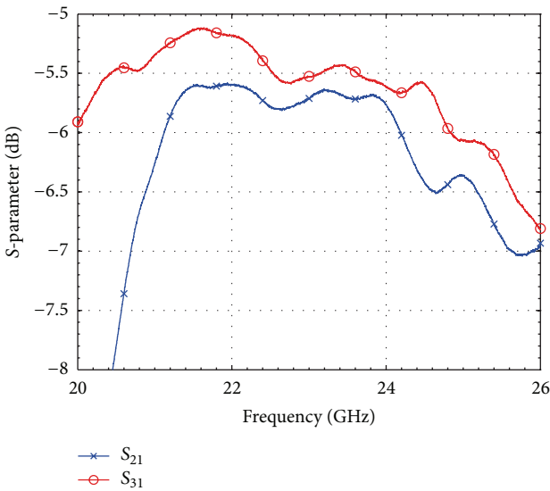
FIGURE 14: Measured transmission coefficient of the hybrid coupler.
