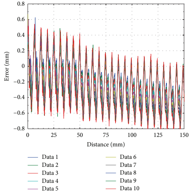
FIGURE 18: Absolute measurement error.
