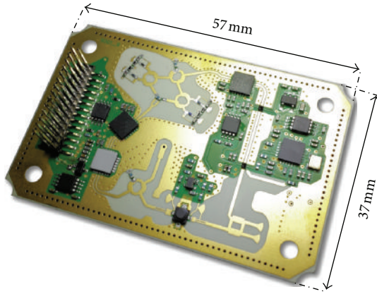
FIGURE 12: Photo of the radar front-end.
