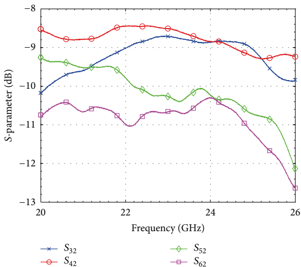
FIGURE 17: Six-port: measured transmission from port 2 to the output ports.
