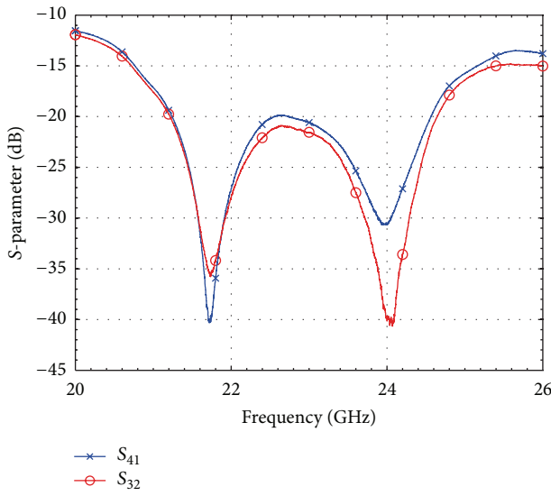
FIGURE 13: Measured S_{41} and S_{32} of the hybrid coupler.
