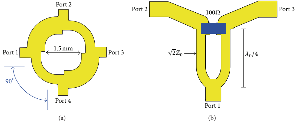
FIGURE 6: Layout of (a) 90° hybrid coupler and (b) Wilkinson power divider.
