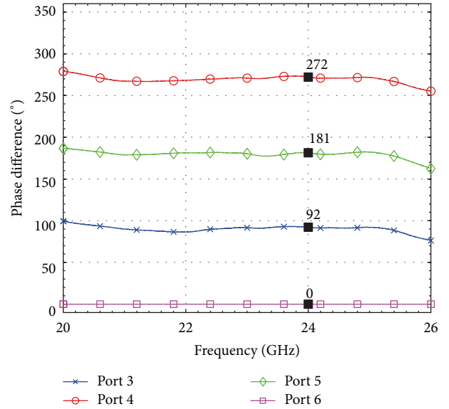
FIGURE 15: Measured normalized phase difference at the output ports of the Six-port network (reference port 6 is set to 0°).
