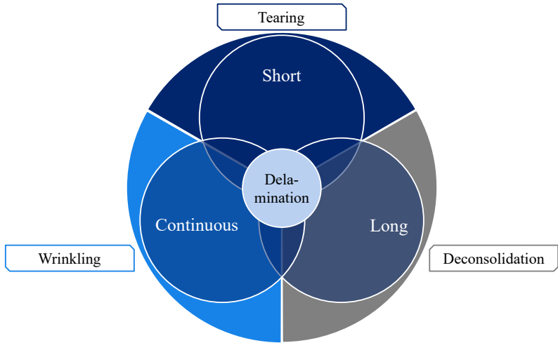
Fig. 3. Failure criteria in FRP ISF and their relation to the reinforcement structure type.
