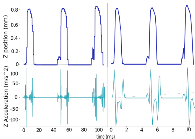
Fig. 3. Extracted z-positions from point cloud and the calculated accelerations based on constant hand speed of 10 (Left) and 100\ \text{mm/s} (Right)
