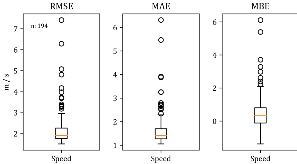
Figure 13: Overall statistical results for wind speed. Speed differences were accounted and are given in m/s. Size of dataset was n = 194.
