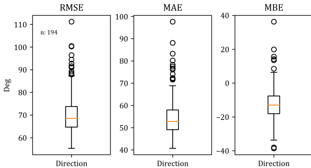
Figure 14: Overall statistical results for wind direction. Direction differences were accounted and are given in ° (degrees). The data resolution of the weather stations was 10°. Size of dataset was n = 194.
