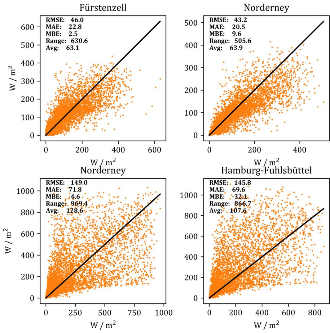
Figure 9: Worst fits of COSMO data and observation data. On top the diffuse irradiation and at the bottom the global irradiation scatter plots. Fürstenzell has both highest RMSE and MAE for DHI. Nordnery has highest |MBE| for DHI and both highest RMSE and MAE for GHI. Hamburg-Fuhlsbüttel has highest |MBE| for GHI.
