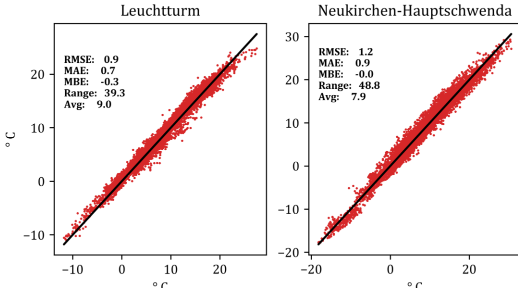
Figure 6: Best fits of COSMO data and observation data. The best in RMSE and MAE is Leuchtturm and in |MBE| Neukirchen-Hauptschwenda.
