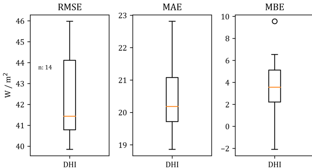
Figure 7: Overall statistical results for diffuse irradiation (ASWDIFD/DHI). Irradiation differences were accounted and are given in W/m^2 . Size of dataset was n = 14 .
