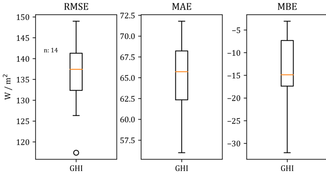
Figure 8: Overall statistical results for global irradiation (ASWDIFD+ASWDIR | GHI). Irradiation differences were accounted and are given in W/m^2 . Size of dataset was n = 14 .
