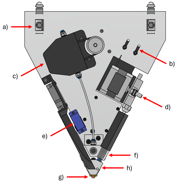
Fig. 7: Front view of the print head design: a) Assembly panel, b) Lift-off guide, c) CCF feeder unit, d) Co-matrix filament extruder, e) Cutting-unit servo motor, f) Cutting-unit/Heat sink combination unit, g) Nozzle, h) Heat block
