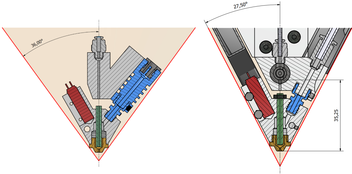
Fig. 3: Cross section of the previous design on the left and redesign described in this work on the right. The two macroscopic optimization parameters of tool angle and minimum cut length are denoted where applicable
