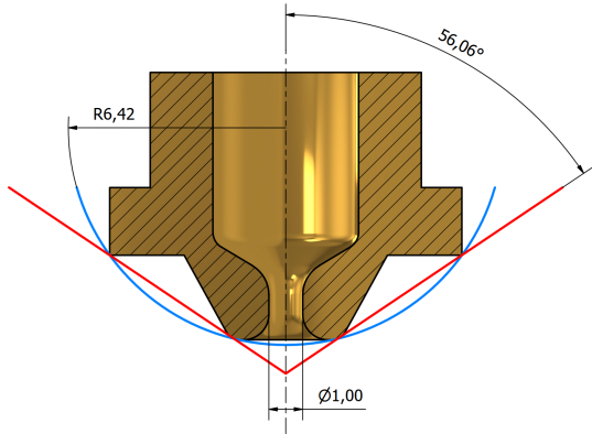
Fig. 2: Microscopic clearance angle, minimum manufacturing radius and bottleneck diameter of the nozzle
