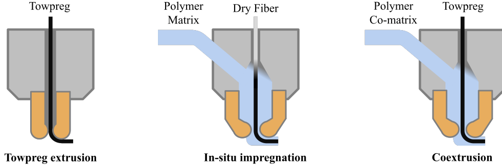
Fig. 1: Extrusion Methods for CFRP. With towpreg extrusion the thermoplastically pre-impregnated filament is directly extruded out of the nozzle; In-situ impregnation denotes the process where dry fiber is impregnated with a thermoplastic matrix inside the print head; Coextrusion refers to the mixing of a towpreg impregnated with a thermoplastic or thermoset matrix with a thermoplastic co-matrix
