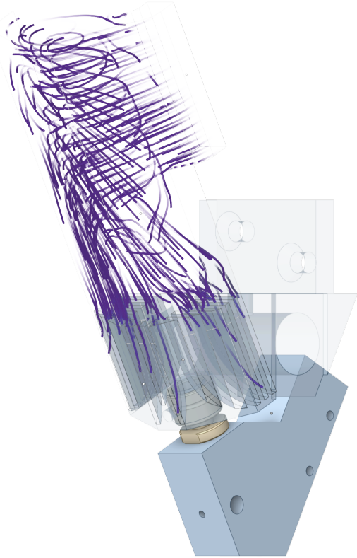
Fig. 6: Visualization of the simulated airflow with streamlines. The rounded bottom vents allow the airflow to flow around the heat block avoiding excessive cooling of the hotend
