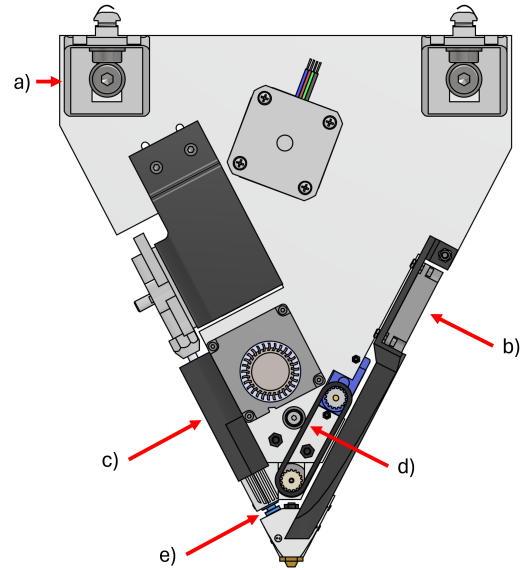
Fig. 8: Back view of the print head design: a) Angle bracket, b) Part Cooling, c) Heat sink cooling, d) Cutting-unit drive belt with tensioner pulley, e) Heat break
