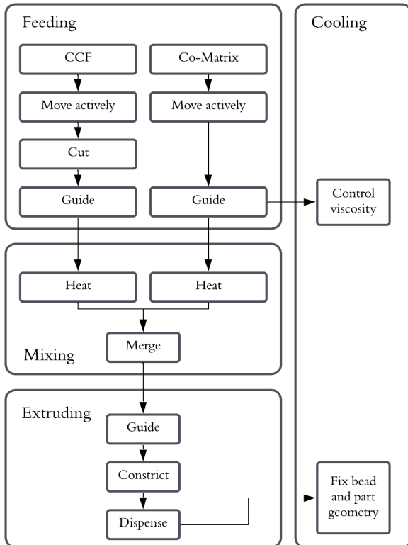
Fig. 4: Functional structure derived from the process analysis. Supergroups are Feeding, Mixing, Extruding and Cooling
