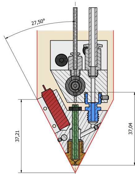
Fig. 10: Version of the proposed printhead with optimized nozzle cross section, compact design and introduction of the additional parameter tool-cone height. This redesign would enable the manufacture of deeper concave features in part and slice geometry
