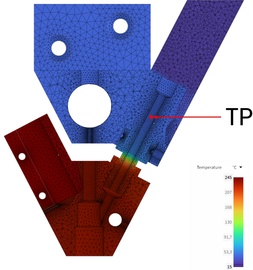
Fig. 5: Thermal simulation with 240°C at the thermistor location and estimated airflow, TP denotes the constant temperature test point. Temperature range indicated by colors
