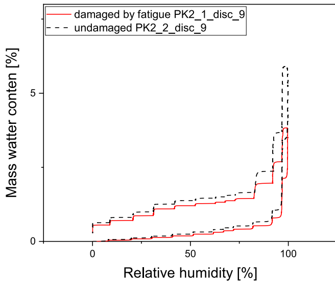
Fig. 19. Changes in mass as a function of relative humidity for the fatigue damaged sample PK2_1 and undamaged sample PK2_2 (disc 9).
