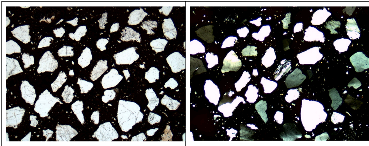
Fig. 5. Thin section, pristine UHPC, picture width 2.45 mm, overview, left without, right with crossed polars. Several quartz grains in matrix.
