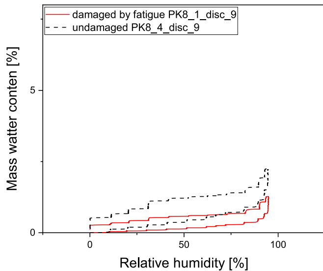
Fig. 21. Changes in mass as a function of relative humidity for the fatigue damaged sample PK8_1 and undamaged sample PK8_4 (disc 9).
