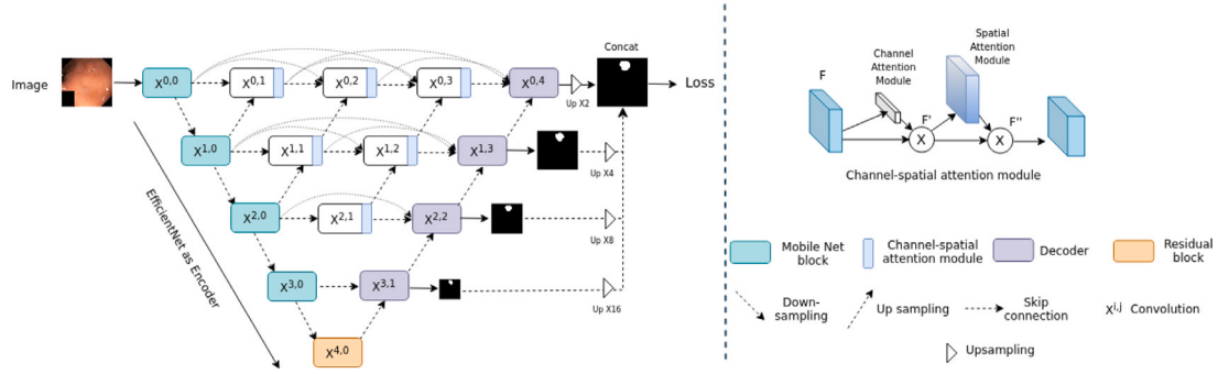
Fig. 4. Overview of the winning solution for the Polyp segmentation task (Task 1) from Team PRML2020GU . The architecture utilizes pre-trained weights from EfficientNet in the encoder. Additionally, it uses dense skip connections, deep supervision and channel-spatial attention for fast convergence and better performance.
