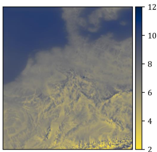
Figure 21: Mean wind speed at 122.32 m distribution 2017 in the data set in m/s. Every pixel represents a ~2.8x2.8 km grid cell.
