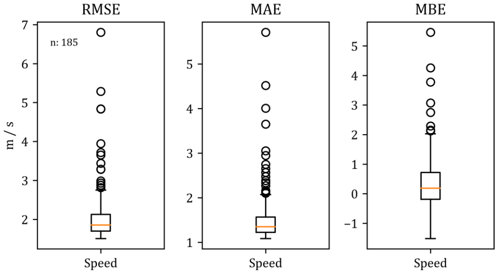
Figure 13: Overall statistical results for wind speed. Speed differences were accounted and are given in m/s. Size of dataset was n = 185.
