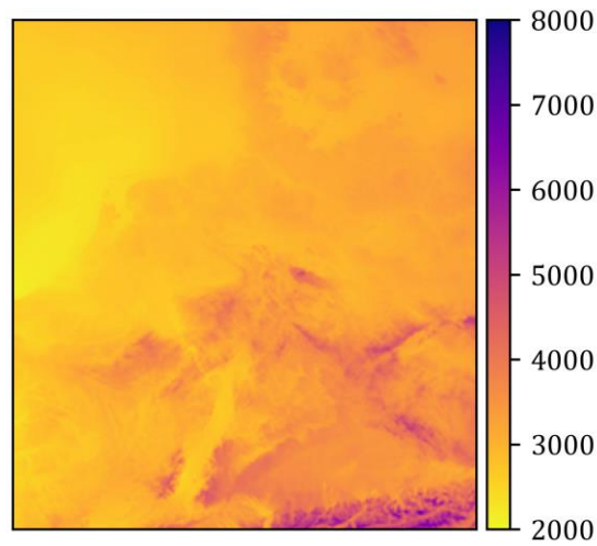
Figure 19: GTZ distribution 2017 in the data set in K. Every pixel represents a ~2.8x2.8 km grid cell.
