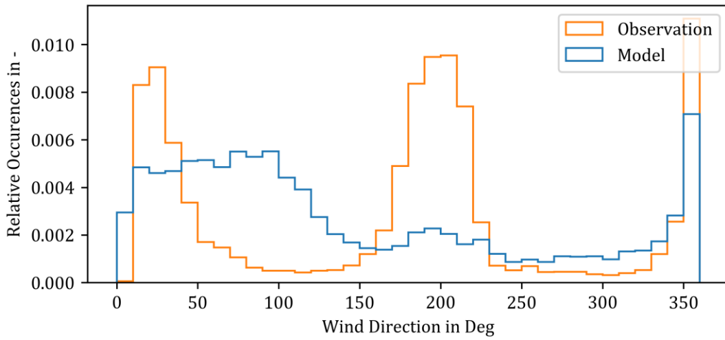
Figure 17: Histogram of worst RMSE fits between model data and weather station's observation data for wind data.
