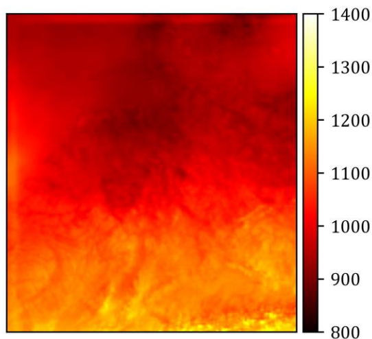
Figure 20: Annual GHI sum distribution 2017 in the data set in kWh/m 2 a. Every pixel represents a ~2.8x2.8 km grid cell.
