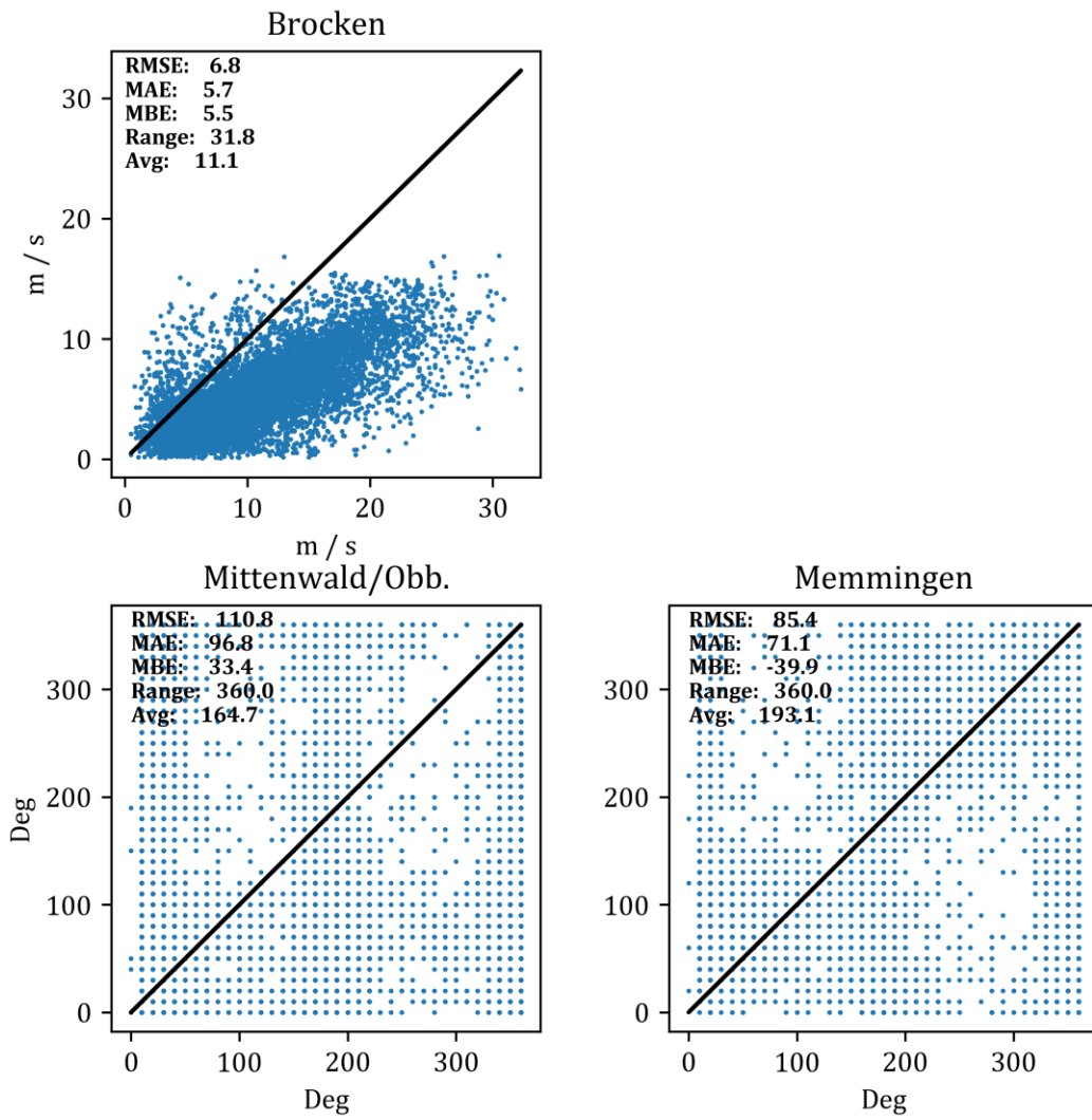
Figure 15: Worst fits of COSMO data and observation data for wind speed, which coincidentally are one of the worst direction results. On top wind speed and at the bottom the wind direction scatter plots. Brocken has all, highest RMSE, MAE and |MBE|, among all weather stations for wind speed, while Mittenwald/Obb. shows highest values in RMSE and MAE and Memmingen in |MBE| for wind direction.
