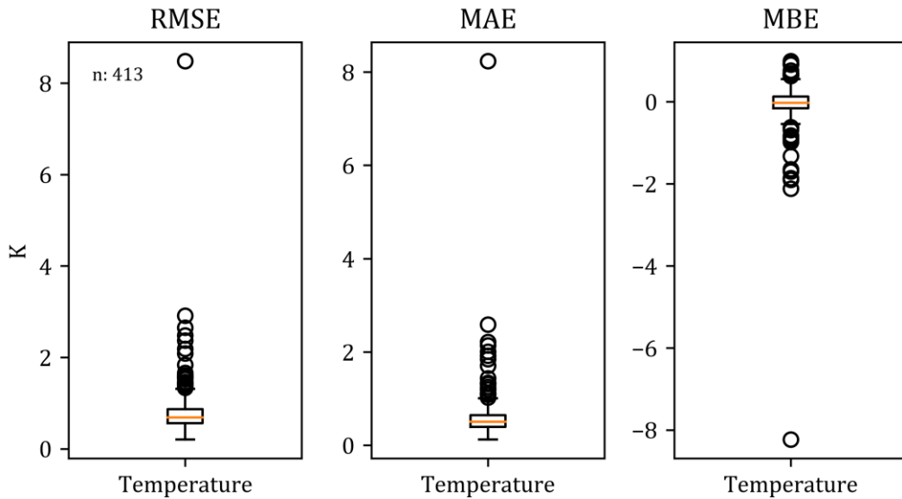
Figure 4: Overall statistical results for temperature. Temperature differences were accounted and are given in Kelvin. Size of dataset was n = 413.
