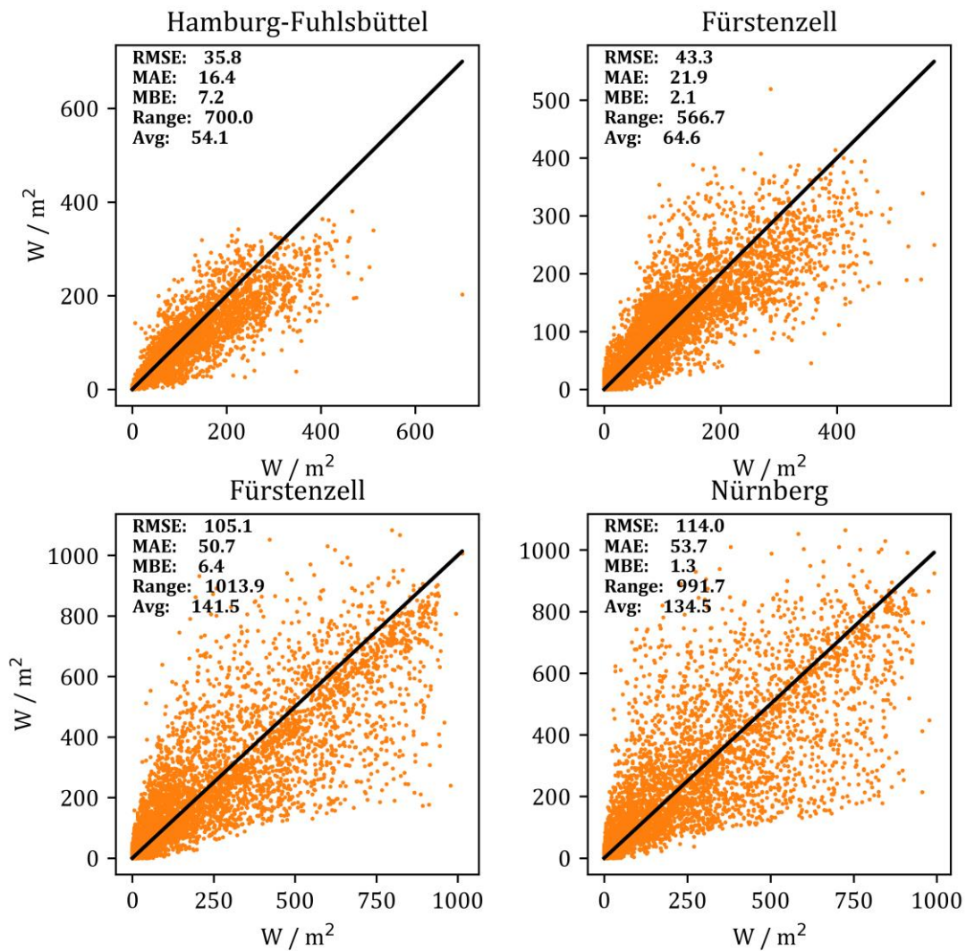
Figure 10: Best fits of COSMO data and observation data. On top the diffuse irradiation and at the bottom the global irradiation scatter plots. Hamburg-Fuhlsbüttel has both lowest RMSE and MAE in DHI, while Fürstenczell has both lowest RMSE and MAE for GHI and lowest |MBE| for DHI. Nürnberg has lowest |MBE| for GHI.
