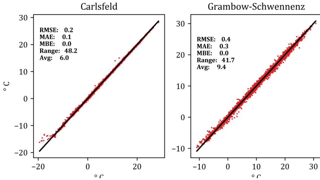
Figure 6: Best fits of COSMO data and observation data. The best in RMSE and MAE is Carlsfeld and in |MBE| Grambow-Schwennenz.
