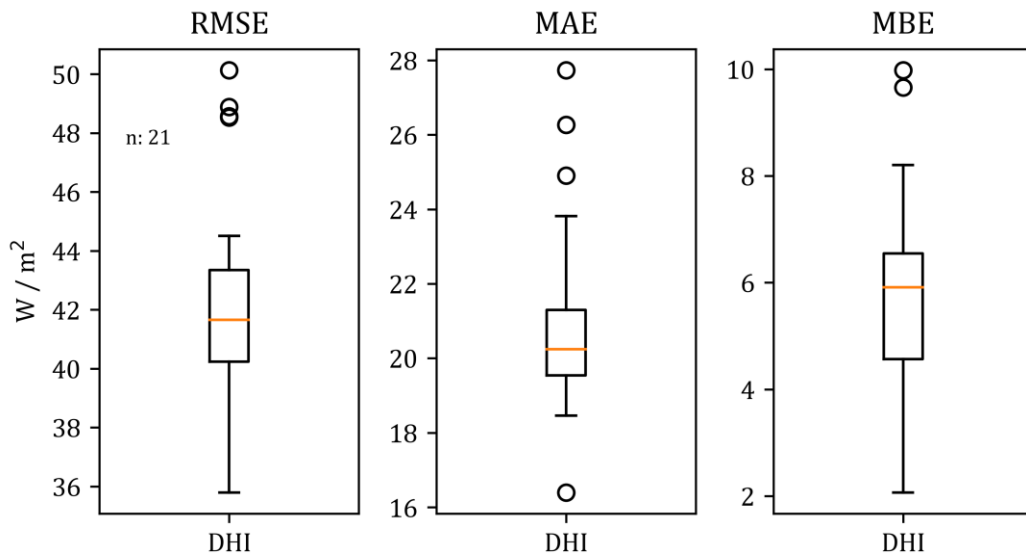
Figure 7: Overall statistical results for diffuse irradiation (ASWDIFD/DHI). Irradiation differences were accounted and are given in W/m^2 . Size of dataset was n = 21 .
