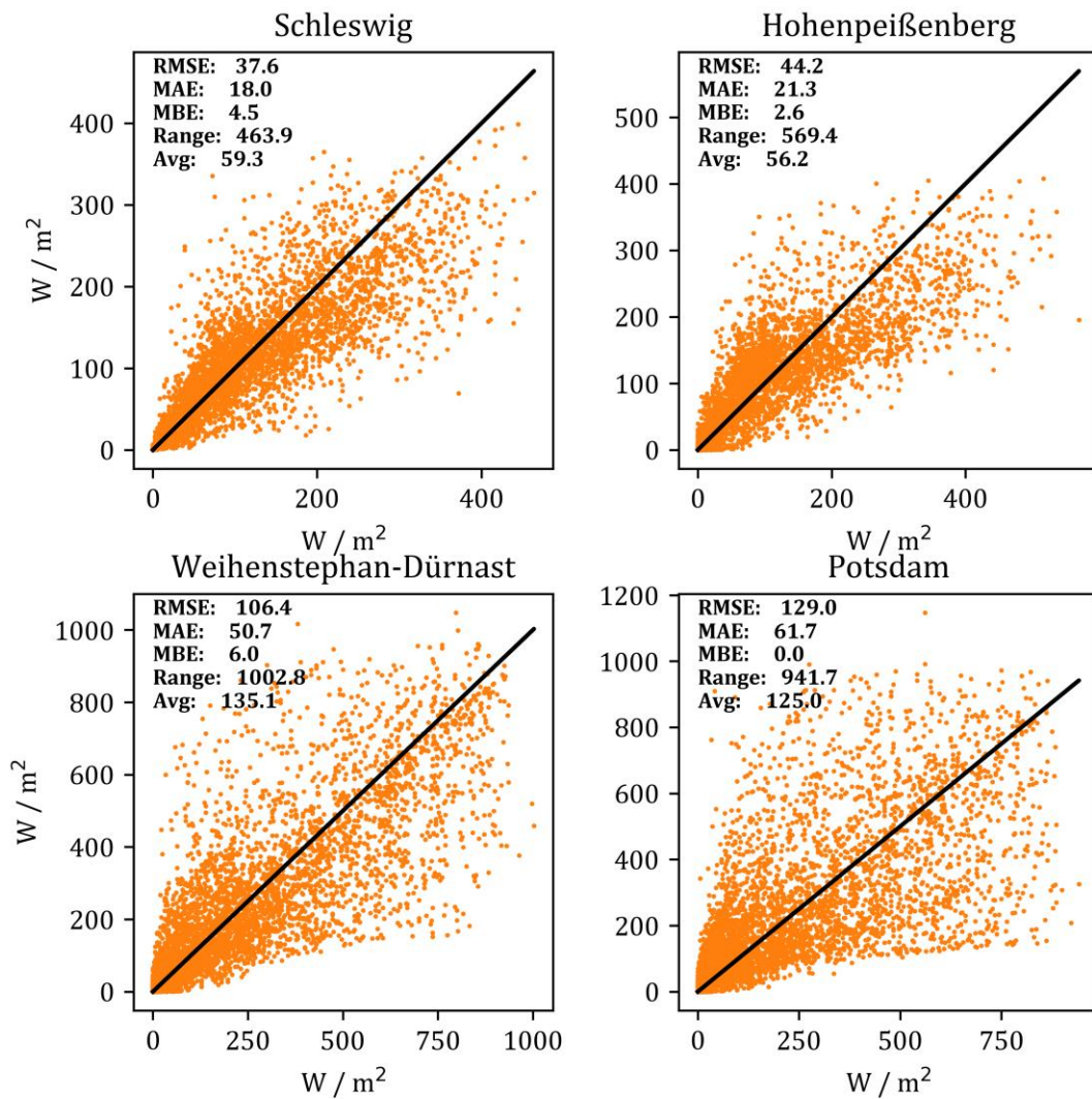
Figure 10: Best fits of COSMO data and observation data. On top the diffuse irradiation and at the bottom the global irradiation scatter plots. Schleswig has both lowest RMSE and MAE in DHI, while Weihenstephan-Dürnast has both lowest RMSE and MAE for GHI. Hohenpeißenberg and Potsdam both have the lowest |MBE|.
