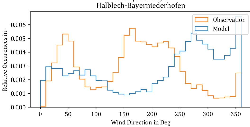
Figure 17: Histogram of worst RMSE fits between model data and weather station's observation data for wind data.
