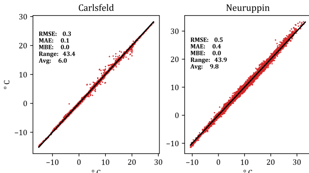
Figure 6: Best fits of COSMO data and observation data. The best in RMSE and MAE is Carlsfeld and in |MBE| Neuruppin.
