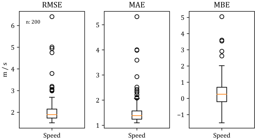
Figure 13: Overall statistical results for wind speed. Speed differences were accounted and are given in m/s. Size of dataset was n = 200.
