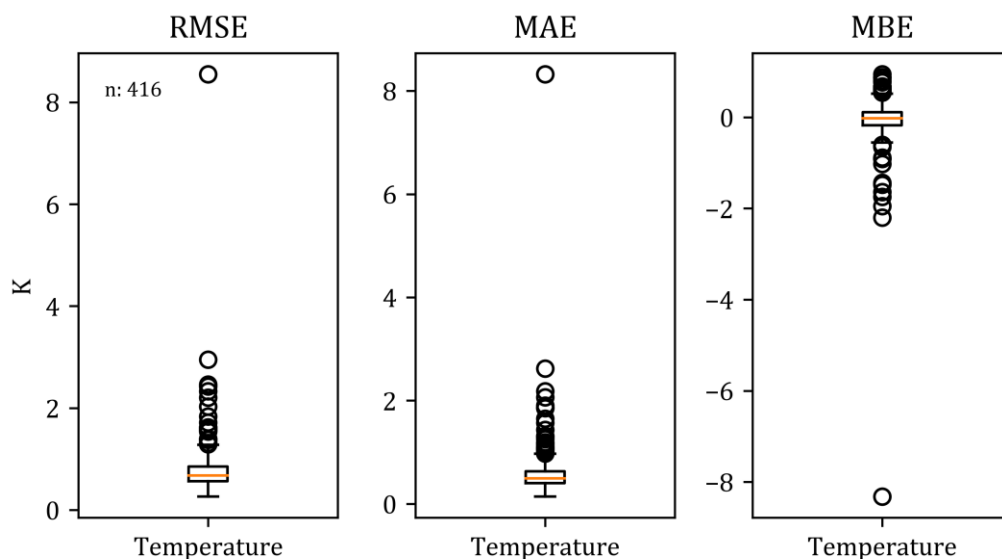
Figure 4: Overall statistical results for temperature. Temperature differences were accounted and are given in Kelvin. Size of dataset was n = 416.
