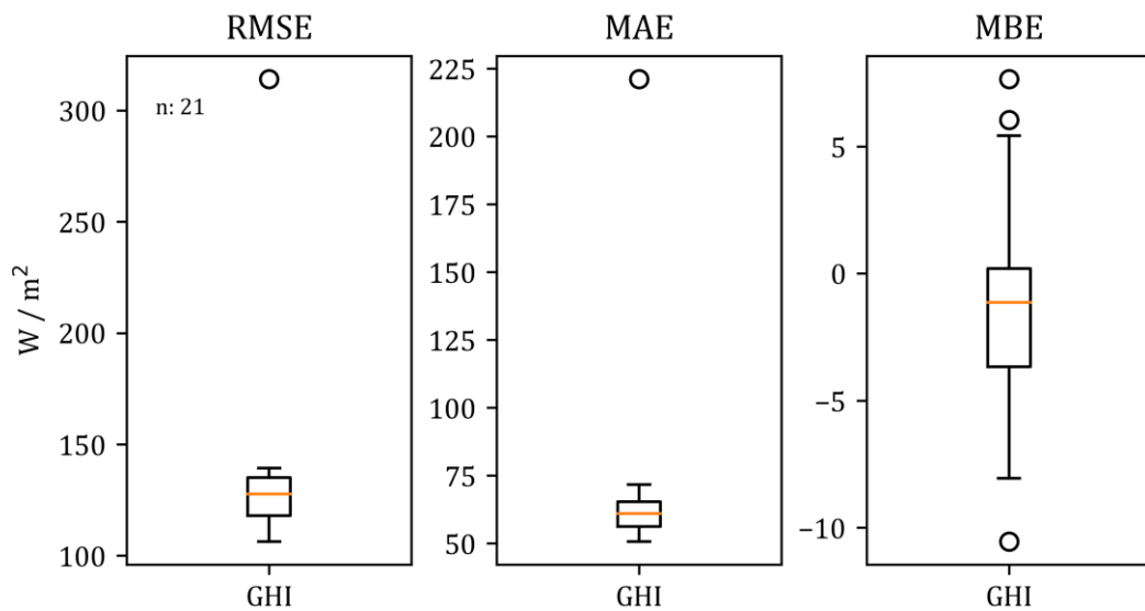
Figure 8: Overall statistical results for global irradiation (ASWDIFD+ASWDIR/GHI). Irradiation differences were accounted and are given in W/m^2 . Size of dataset was n = 21 .
