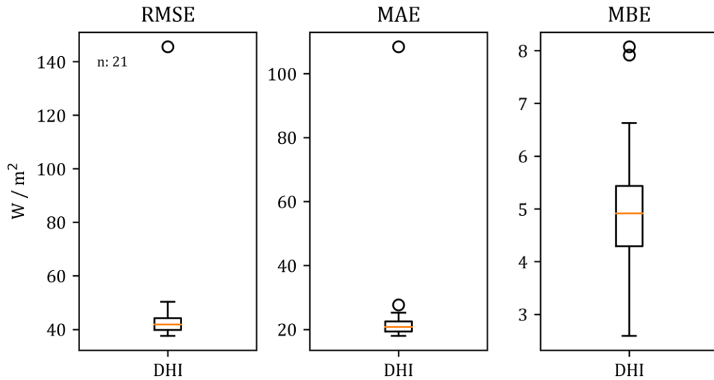
Figure 7: Overall statistical results for diffuse irradiation (ASWDIFD/DHI). Irradiation differences were accounted and are given in W/m^2 . Size of dataset was n = 21 .
