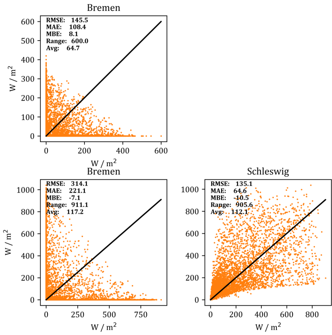
Figure 9: Worst fits of COSMO data and observation data. On top the diffuse irradiation and at the bottom the global irradiation scatter plots. Bremen has both highest RMSE and MAE in DHI and GHI as well as highest |MBE| for DHI and Schleswig has the highest |MBE| for GHI.
