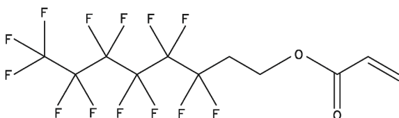
Fig. 3. Molecular structure of 1H,1H,2H,2H-perfluorooctylacrilate.
