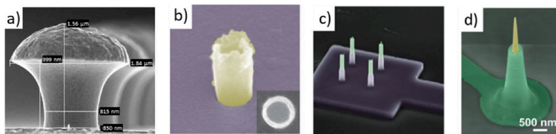
Figure 1. Nanoelectrodes made with different fabrication approaches and shapes. (a) Scanning electron microscopy (SEM) image of so-called gold-spine electrodes (adapted with permission from Hai et al. 67 Copyright 2009 The Royal Society). The height of the structure is 1.56 \mu\text{m} . (b) SEM image of an iridium oxide nanotube electrode (adapted with permission from Lin et al. 74 Copyright 2014 Springer Nature Limited). (c) SEM image of core-shell-type nanowires connected toward external contacts with encapsulated conductive lines (adapted with permission from Casanova et al. 75 Copyright 2018 IOP Publishing Ltd). (d) SEM image of a silicon-based ultrasharp nanowire with an exposed Pt tip (adapted with permission from Liu et al. 76 Copyright 2022 Wiley-VCH).
