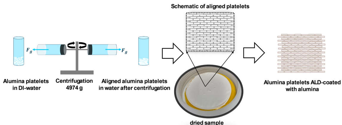
Fig. 1. Schematic drawing shows an overview of the fabrication process involving centrifugation of alumina platelets as brick material to form the to-be-coated skeleton, followed by ALD coating of aluminum oxide to serve as the mortar material resulting in ceramic-ceramic nacre-like composites.
