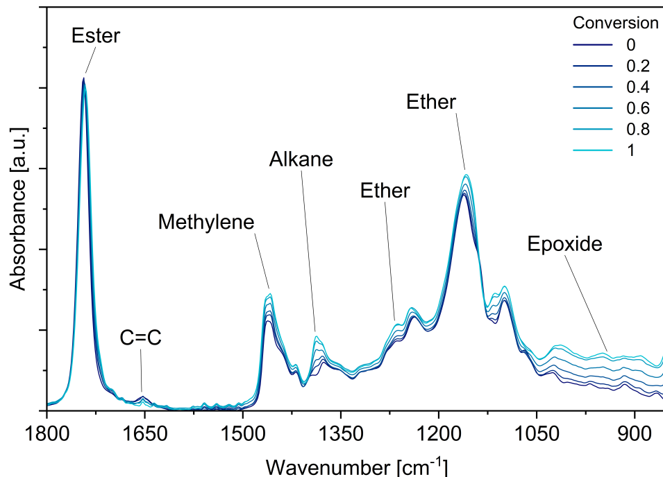
Figure 5.39 Overlay of mixture ATR-FTIR spectra of LO and ELO at different conversion. Scan resolution: 2\text{ cm}^{-1} , Scan number: 50, rubberband baseline correction (64 nodes, 10 iterations), min-max normalization.
