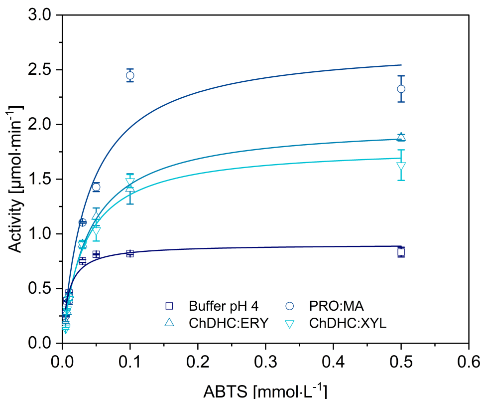
Figure 5.29 Michaelis–Menten kinetics of LacF for ABTS oxidation in 0.1 \text{ mol} \cdot \text{L}^{-1} citrate-phosphate buffer (pH 4) and selected DES–water mixtures. Curves represent non-linear fits.
