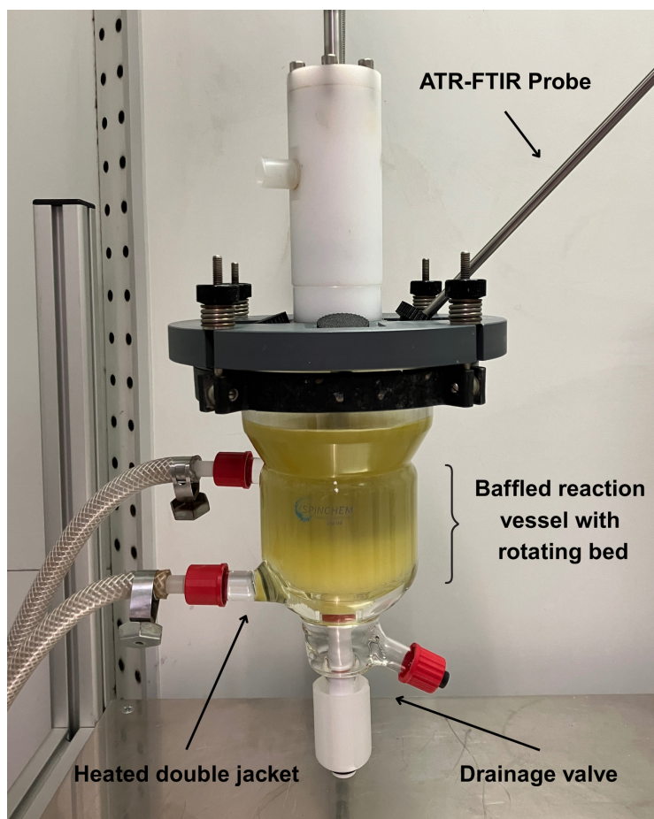
Figure 5.47 Photograph of reaction setup employing the SpinChem ® V2 RBR (SpinChem ® , Umeå, Sweden) system with inline ATR-FTIR acquisition.
