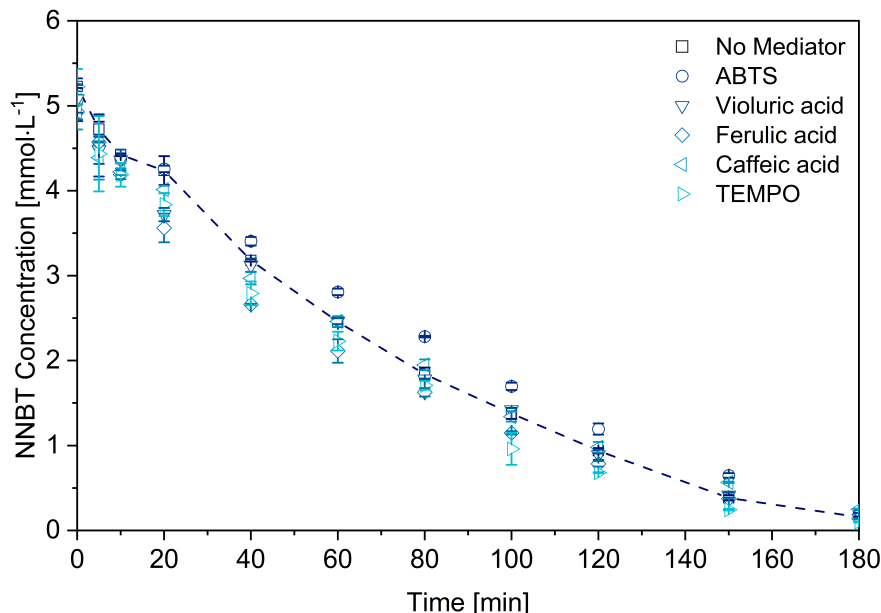
Figure 5.10 NNBT oxidation over time in the presence of various redox mediators. Dotted line inserted to enhance readability. 10 mL reaction volume, 5 \text{ mmol} \cdot \text{L}^{-1} NNBT, 1.5 \text{ mmol} \cdot \text{L}^{-1} mediator, 0.1 \text{ U} \cdot \text{mL}^{-1} laccase, 0.1 \text{ mol} \cdot \text{L}^{-1} citrate-phosphate buffer (pH 4.5), 30^\circ\text{C} , 750 rpm, 200 \mu\text{L} sample was inhibited by 5 \mu\text{L} 0.05 % \text{NaN}_3 , remaining NNBT concentration was determined after pH adjustment to 7 and 1:1 extraction with EtOAc via GC-FID.
