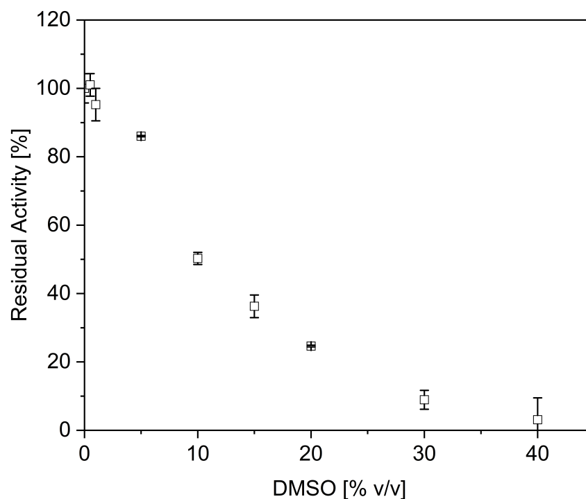
Figure A.1 DMSO tolerance of laccase from Funalia troglia (LacF) in 0.1 \text{ mol} \cdot \text{L}^{-1} aqueous citrate-phosphate buffer at pH 4. Activity determined according to Section 4.5.
