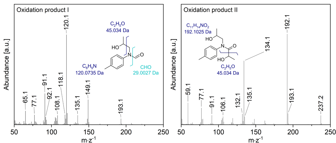
Figure 5.17 Fragmentation pattern of oxidation products I and II from NNBT as identified in the TIC. Assignments are based on elemental composition and structure-supported fragmentation. Proposed fragments are color-coded.
