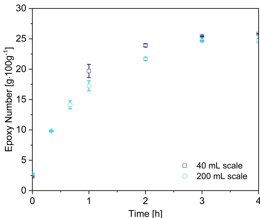
Figure 5.48 Chemoenzymatic epoxidation of LO to ELO in toluene with Novozyme ® 435 and BA in SpinChem ® V2 rotating bed reactor, 26.8 g LO in 200 mL toluene, 50 °C, 6% (w·w oil -1 Novozyme ® 435, 0.5 mol BA :C=C, 1.75 mol H 2 O 2 :C=C, 1000 rpm overhead stirring. EN determined via non-aqueous titration according to Section 4.13.
