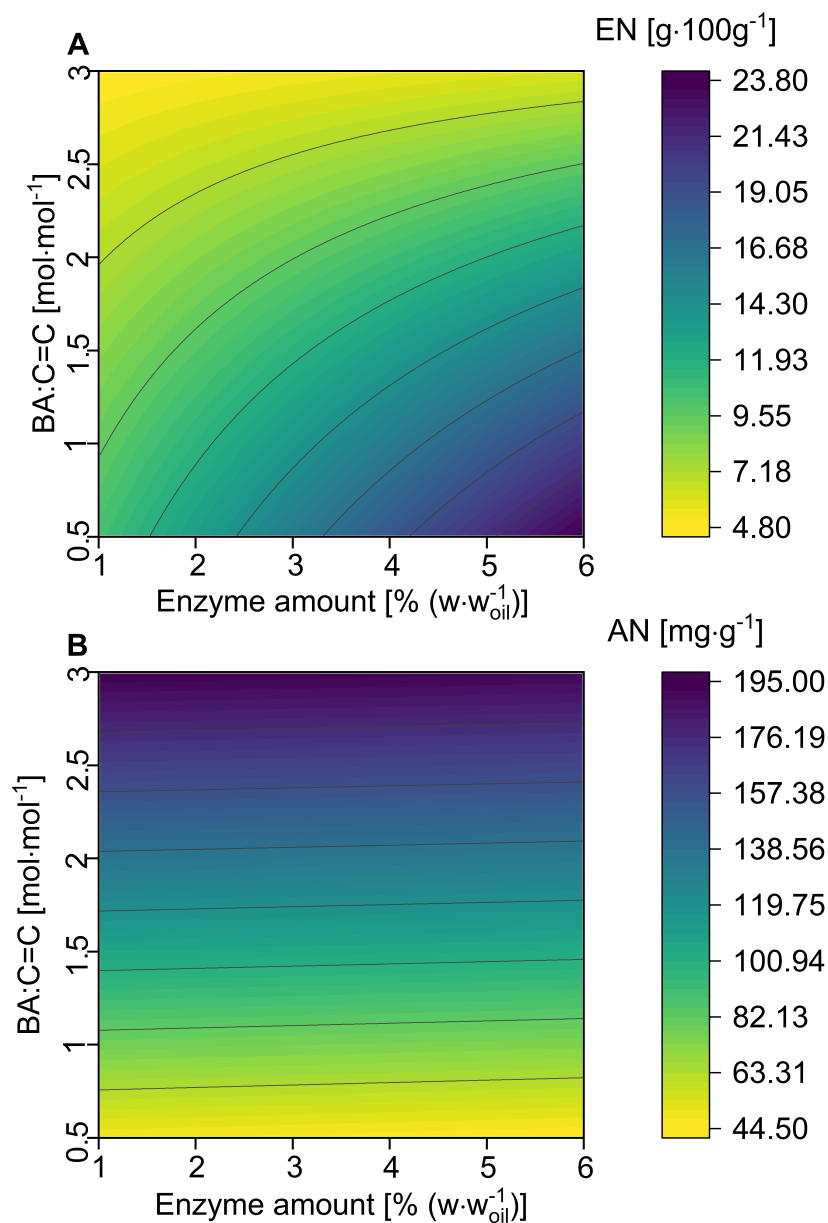
Figure 5.45 Contour plots showing the effect of enzyme concentration and BA:C=C ratio on epoxy number (A) and acid number (B) at fixed \text{H}_2\text{O}_2/\text{C}=\text{C} ratio. A high EN and low AN indicate favorable process conditions.
