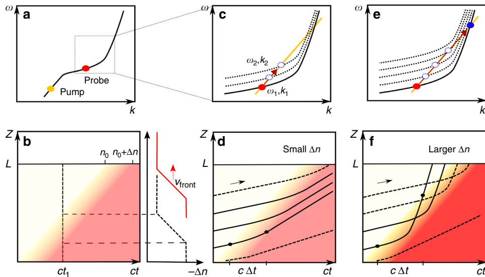
Fig. 4 Schematic representations of the induced interband and intraband photonic transitions. a Schematic representation of the dispersion band of our PhC waveguide. Red and orange dots indicate the locations of the input probe wave packets and the pump pulse, respectively. b Spatiotemporal change of \Delta n . The red filling colour indicates the z -coordinate range of the waveguide where the refractive index has been switched already (switched zone). The graded reddish area indicates the fact that the time function of the pump pulse power has a finite steepness, thus the refractive index front is gradual in any position as the pump pulse transforms the waveguide medium. The two horizontal dotted lines represent the rising length of the index front. The velocity of the refractive index front, indicated in b , d , f as the slope of any line of equal reddish colour tone in the graded part, is the same as the group velocity of the pump pulse thus equal to the slope of the band at pump frequency. c , e show the dispersion bands and the corresponding interband and intraband photonic transitions of the input probe caused by insufficient (dashed blue dots) and by sufficient (solid blue dots) values of \Delta n , respectively. d , f Schematic illustrations of the probe wave signal trajectories for the induced transitions in c , e , respectively. Black lines in d , f represent wave packets of the CW input probe. Solid lines illustrate the wave packets which undergo complete interband d and intraband f transitions, while the dashed lines depict the wave packets which only undergo incomplete transitions. The black dots in d , f mark the points where the wave packet enters and exits the front
