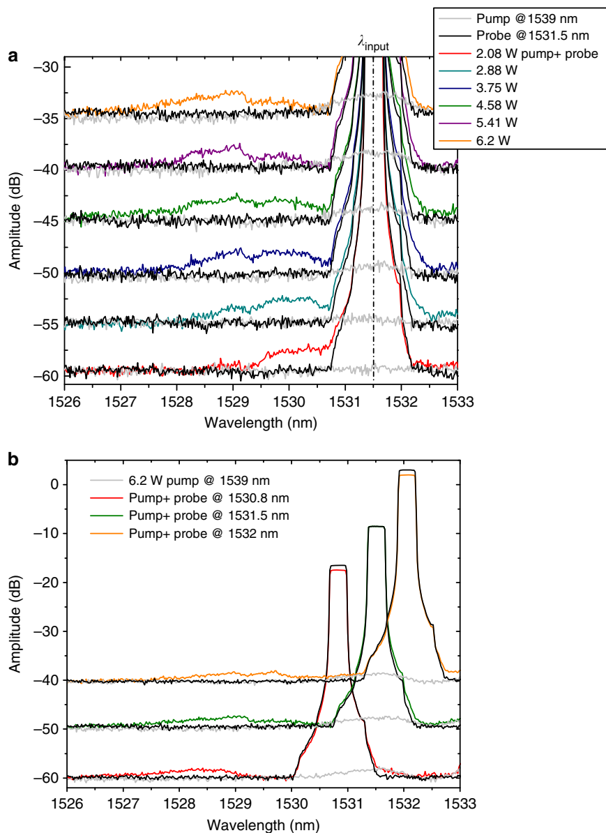
Fig. 3 Experimental spectra recorded at the output of our 396 \mu\text{m} -long slow light silicon PhC waveguide. a Pump pulse peak power-dependent output spectra for the blue-shifted light of an input probe wave at a wavelength of 1531.5 nm. Shown is the spectrum of the CW probe that has not interacted with the pump pulses (black traces), the spectrum of the pump pulses alone (grey traces), and shown are the spectra of both the pump pulses and the CW probe (other colours). b Spectra for different input probe wavelengths. The different curves in a , b are shifted by 5 and 10 dB, respectively for clarity, the noise level corresponds to -60 dBm
