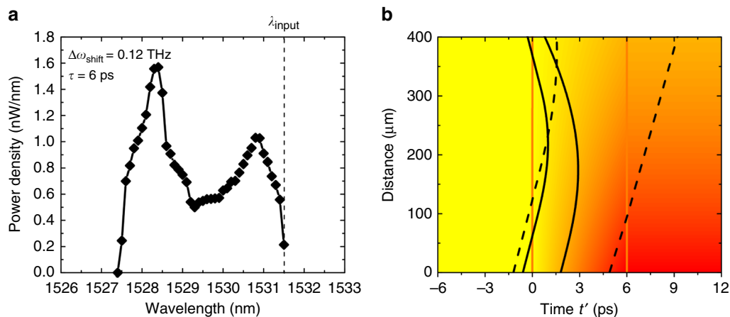
Fig. 5 Simulation of the FC front interaction with CW probe wave packets via ray tracing. a Wave packets average power spectrum for 6 \mu\text{W} average power of the CW probe at 1531.5 nm, rising time of the front of 6 ps, and initial band shift \Delta\omega_{\text{shift}} of 0.12 THz. Other parameters are listed in the Supplementary Note 6. b The trajectories of the probe wave packets with respect to the front velocity. The two vertical orange lines represent the extent of the index front with a rise time of 6 ps, while the shading represents the refractive index front as it exponentially decays during propagation inside the waveguide. Solid black lines represent those wave packets that undergo complete transitions, while the dashed lines depict the wave packets which only undergo incomplete transitions
