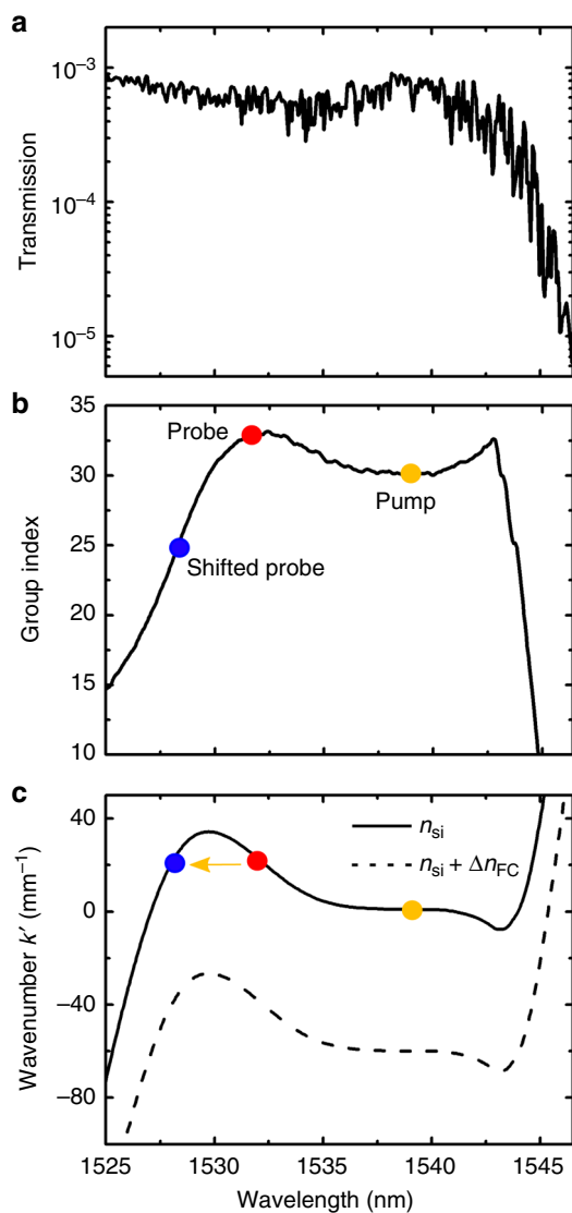
Fig. 2 Characteristics of the fabricated slow light silicon PhC waveguide. a Linear transmission and b measured group index. c The calculated dispersion band from the measured group index in b . The wave vector corrected by the slope of the pump group velocity is presented. Due to very small band diagram shift the curves cannot be presented in the original form similar to Fig. 1a. Solid curve represents the original dispersion band of waveguide mode with refractive index n_{si} , while the dashed curve indicates the waveguide mode with refractive index change of \approx -3 \times 10^{-3} . Dots indicate the locations of the input wavelengths of probe wave (red dot), pump pulse (orange dot) and the expected output wavelength of the shifted probe wave (blue dot) after the intraband transition took place. The orange line represents the phase continuity line with a slope equal to the travelling velocity of the pump pulse. Due to the slope correction, this phase continuity line now appears horizontal
