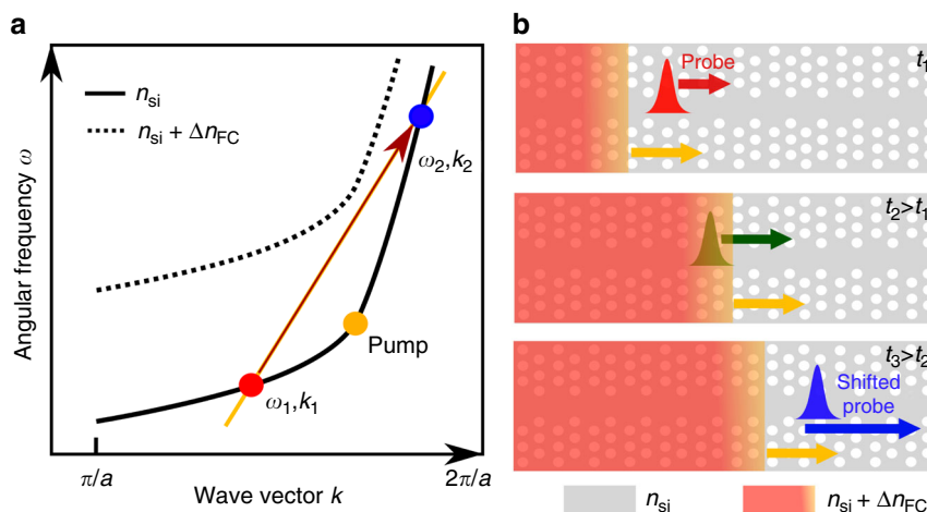
Fig. 1 Schematic of the interaction between front and probe. a Schematic representation of an intraband indirect photonic transition in a slow light silicon PhC waveguide. The solid curve represents the dispersion band of waveguide mode in the ground state (with refractive index n_{\text{si}} ), while the dashed curve indicates the switched state with refractive index n_{\text{si}} + \Delta n_{\text{FC}} . We use the PhC band with positive group velocity to represent the dispersion relationship. The orange line represents the phase continuity line with a slope equal to the group velocity of the pump pulse set at the knee of the dispersion band (orange dot). The red and blue dots indicate the initial (slow mode) and final (fast mode) states of a probe wave, respectively. b Schematic of the experiment. A pump pulse generates FCs in the silicon by TPA and, consequently, induces a change of refractive index which propagates with the velocity of the pump pulse. The region with the red colour gradient corresponds to the rising edge of the front. The orange arrow indicates the velocity of the pump pulse, while red, green and blue arrows indicate the velocities of a wave packet of the probe at different times, respectively
