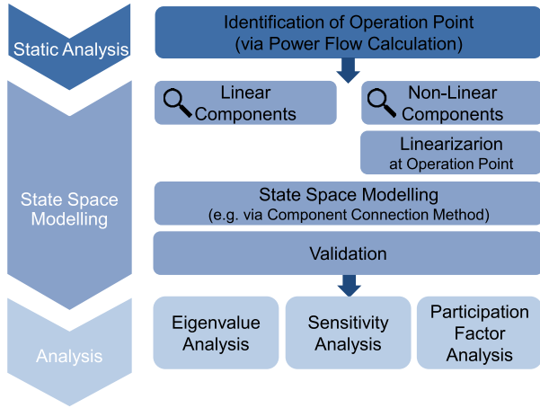
FIGURE 10. General procedure for small signal stability analysis with eigenvalue, sensistivity, and participation factor analysis.
