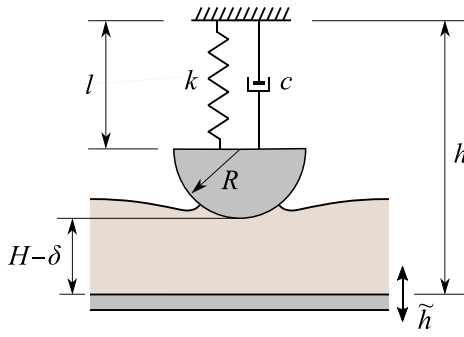
Fig. 1. Schematic of the adhesive contact between a hemispherical probe and an elastic sample: Dynamic equilibrium.
