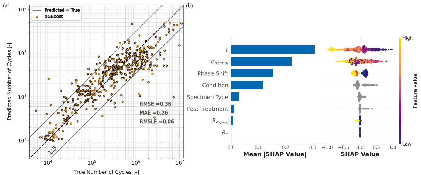
Fig. 11. Predicted number of cycles from randomly shuffled 14-fold cross-validation using only stress-related features with the XGBoost algorithm versus the true number of cycles from fatigue tests (a). SHAP analysis of the corresponding predictions (b).
