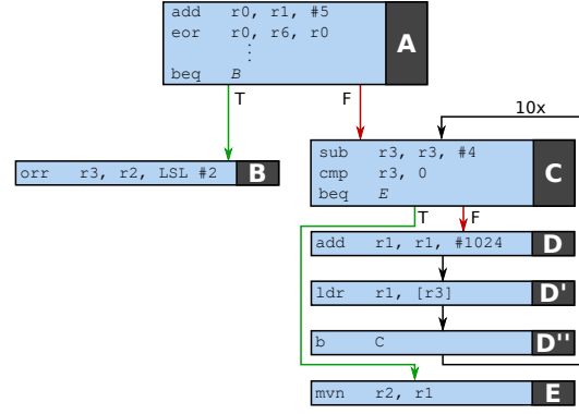
■ Figure 8 Exemplary CFG from Figure 5 with sub basic block splitting.
