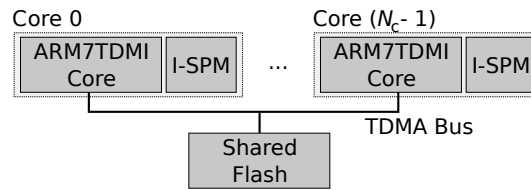
■ Figure 1 Overview of the proposed multicore architecture.
