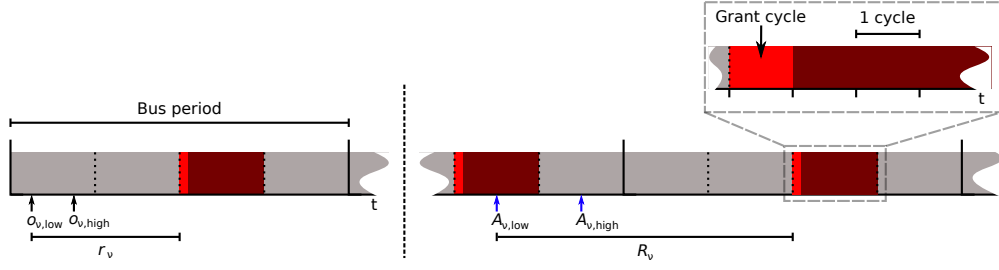
■ Figure 7 Two exemplary bus offset intervals o_{\nu} and A_{\nu} in regard to the bus schedule. The bus slot of the third core is highlighted, as well as the grant cycle during which an access can be issued.
