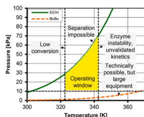
Fig. 8. Reaction scheme (top left), operating window (bottom left) demonstrating suitable operation conditions in respect to pressure and temperature, and process concept (right a) with catalytic packings (right b and c) for the immobilization of enzymes in the reactive zone for the transesterification of ethyl butyrate with butanol, where b has coated packings and c has bags for immobilised enzymes introduced in the packings. Reproduced from [85] with permission from Elsevier.
