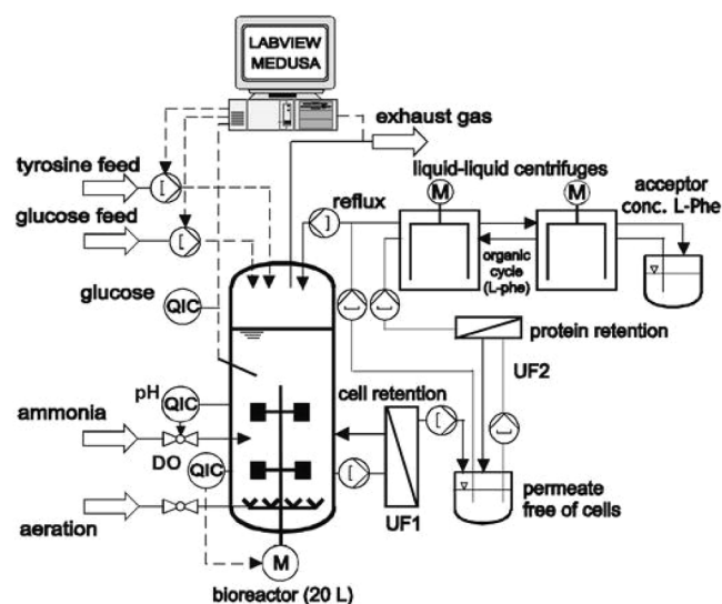
Fig. 11. Process scheme of a phenylalanine fermentation with integrated product separation. Reproduced from [117], with permission from SNCSC.
