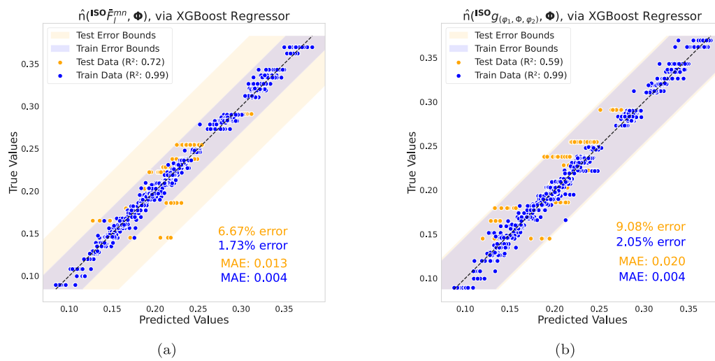
Fig. C.22. True and predicted values of Strain Hardening Exponent, n , for XGBoost regressor using input features (a) \text{ISO}\hat{F}^{mn} , and (b) \text{ISO}\hat{g}_{(\phi_1, \phi, \phi_2)} with input set \Phi at scale = 100 \mu\text{m} .
