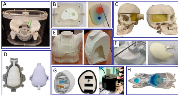
Fig. 4. Selection of 3D printed phantoms. A Pelvic phantom from [4], B Prostate mold and prostate phantom from [4], C Head phantom from [19], D Bladder mold and bladder phantom adapted from [4, 20], E Sliced thorax phantom from [17], F Lung phantom from [15], G Arm slice phantom from [21], H Mouse phantom from [22].
