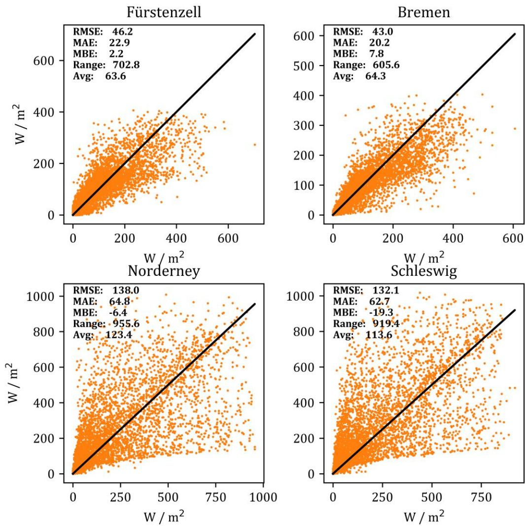
Figure 9: Worst fits of COSMO data and observation data. On top the diffuse irradiation and at the bottom the global irradiation scatter plots. Fürstentzell has both highest RMSE and MAE for DHI, and Norderney the same for GHI. Bremen and Schleswig have the highest |MBE| for DHI and GHI respectively.
