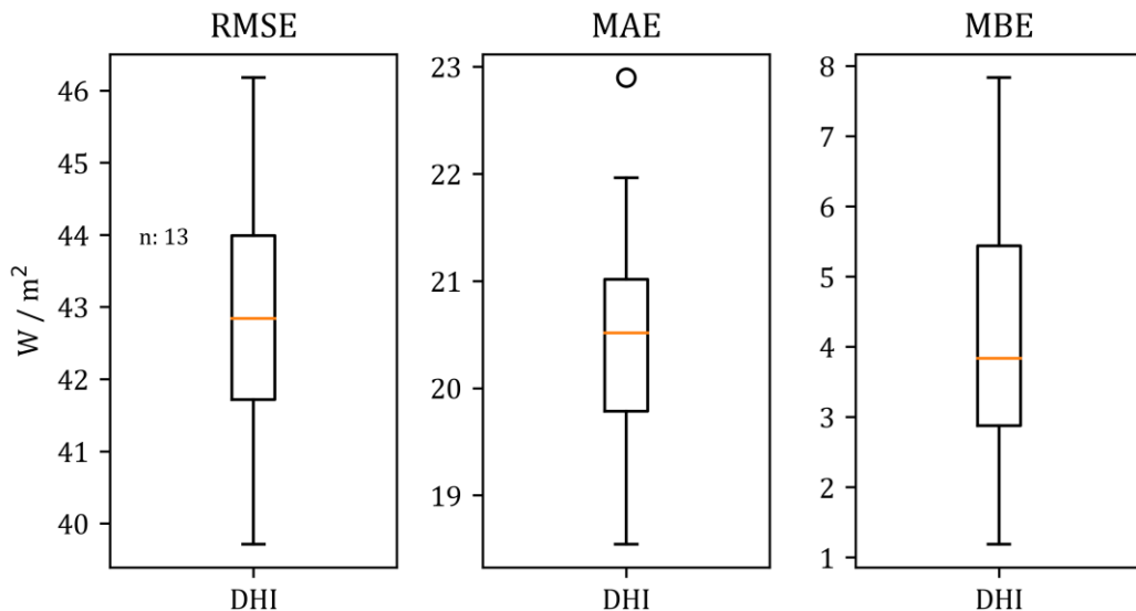
Figure 7: Overall statistical results for diffuse irradiation (ASWDIFD/DHI). Irradiation differences were accounted and are given in W/m^2 . Size of dataset was n = 13 .
