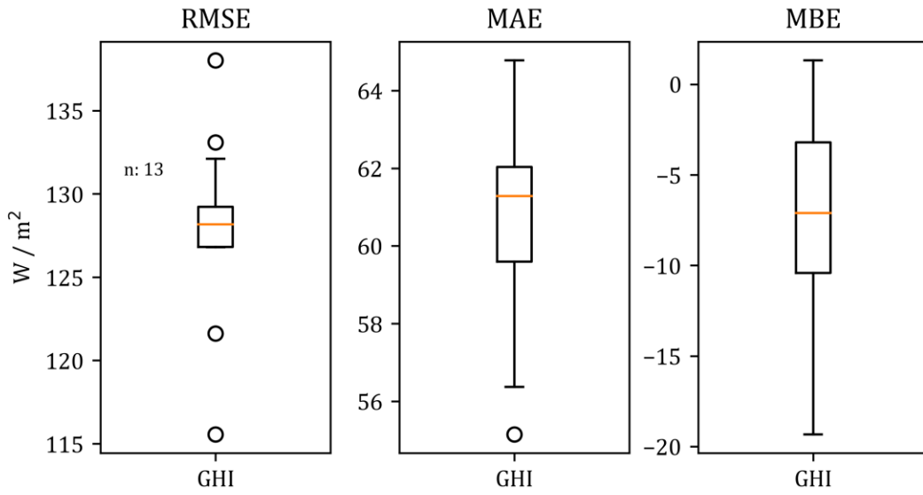
Figure 8: Overall statistical results for global irradiation (ASWDIFD+ASWDIR | GHI). Irradiation differences were accounted and are given in W/m^2 . Size of dataset was n = 13 .
