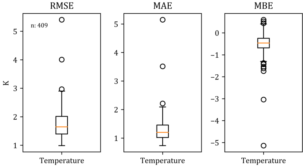
Figure 4: Overall statistical results for temperature. Temperature differences were accounted and are given in Kelvin. Size of dataset was n = 409.
