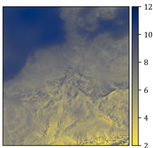
Figure 21: Mean wind speed at 122.32 m distribution 2011 in the data set in m/s. Every pixel represents a ~2.8x2.8 km grid cell.
