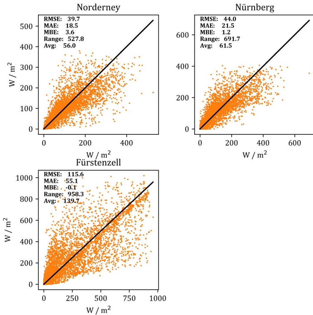
Figure 10: Best fits of COSMO data and observation data. On top the diffuse irradiation and at the bottom the global irradiation scatter plots. Norderney has both lowest RMSE and MAE in DHI, while Fürstenzell has all lowest RMSE, MAE, and |MBE| for GHI. Nürnberg has the lowest |MBE| for DHI.
