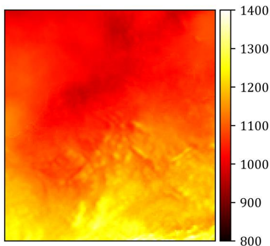
Figure 20: Annual GHI sum distribution 2011 in the data set in kWh/m 2 a. Every pixel represents a ~7x7 km grid cell.
