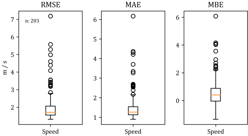
Figure 13: Overall statistical results for wind speed. Speed differences were accounted and are given in m/s. Size of dataset was n = 203.
