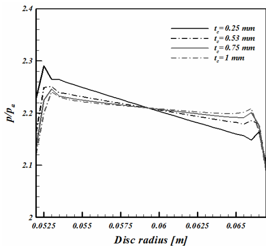
Figure 6. Variation of the normalized contact pressure with disc radius using different friction facing thicknesses ( f.s = 5 )
