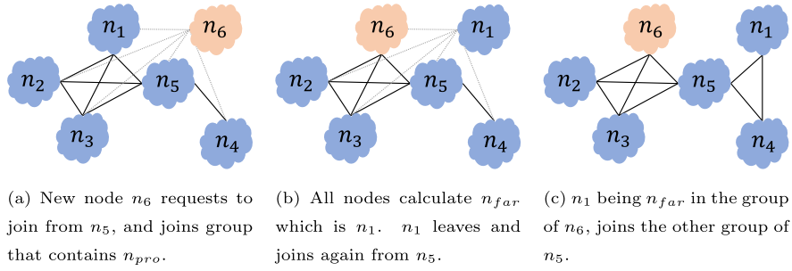
Fig. 7. Example of the process of FPI step-by-step (for S = 4 ).
