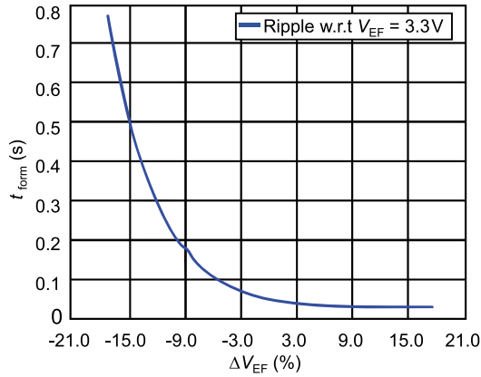
Fig. 16. EF time t_{\text{form}} as function of change in EF voltage \Delta V_{\text{EF}} simulated using HfO 2 memristor.
