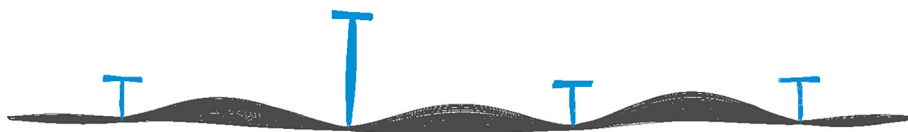
Fig. 11. Example of the measured imperfections applied to the FE model (plate and longitudinal stiffeners, values magnified by a factor of 10 for clarity).
