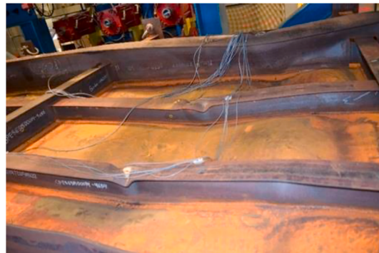
Fig. 8. View of the final deformed structure shape in Section 2 illustrating the plate buckling, stiffener buckling, and girder tripping buckling modes.
