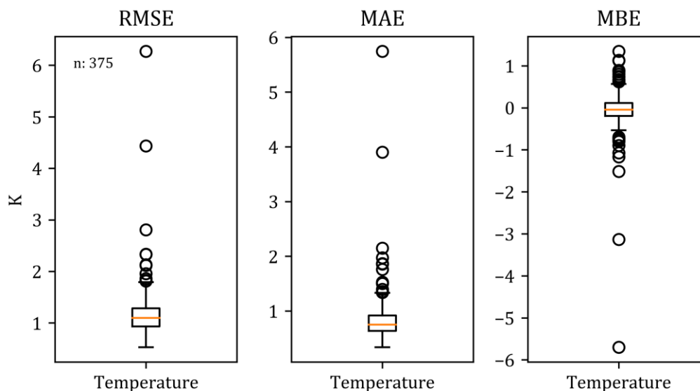
Figure 4: Overall statistical results for temperature. Temperature differences were accounted and are given in Kelvin. Size of dataset was n = 375.
