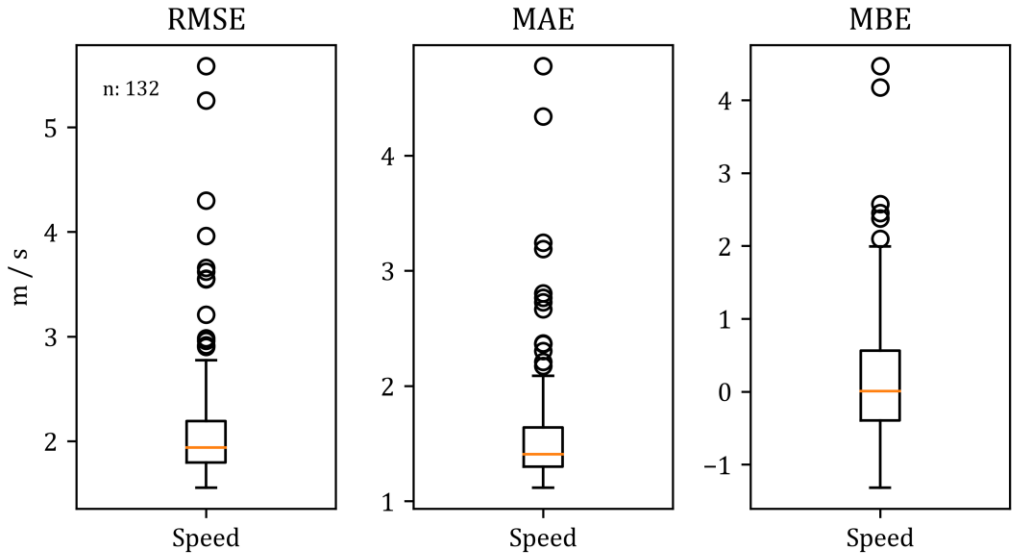
Figure 7: Overall statistical results for wind speed. Speed differences were accounted and are given in m/s. Size of dataset was n = 132.
