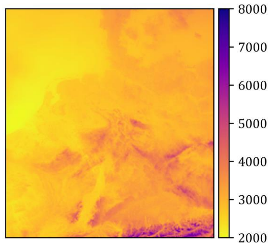
Figure 13: GTZ distribution 2007 in the data set in K. Every pixel represents a ~2.8x2.8 km grid cell.
