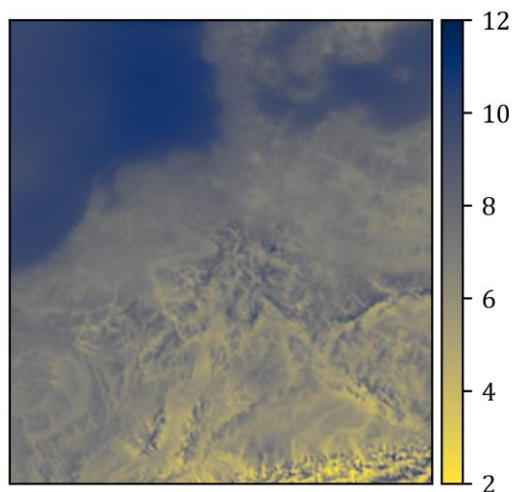
Figure 14: Mean wind speed at 122.32 m distribution 2007 in the data set in m/s. Every pixel represents a \sim 2.8 \times 2.8 km grid cell.
