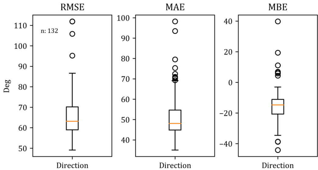
Figure 8: Overall statistical results for wind direction. Direction differences were accounted and are given in ° (degrees). The data resolution of the weather stations was 10°. Size of dataset was n = 132.
