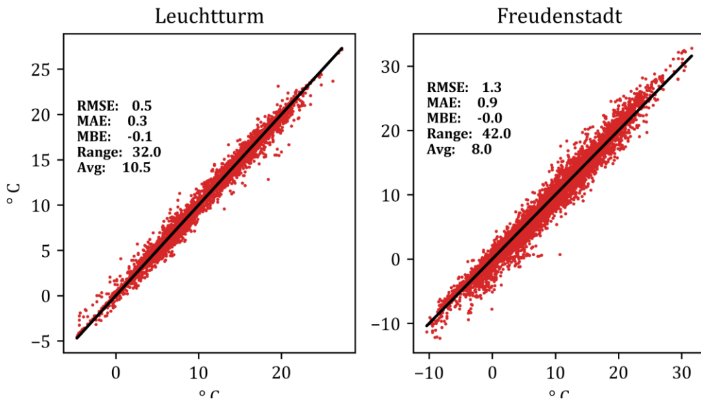
Figure 6: Best fits of COSMO data and observation data. The best in RMSE and MAE is Leuchtturm and in |MBE| Freudenstadt.
