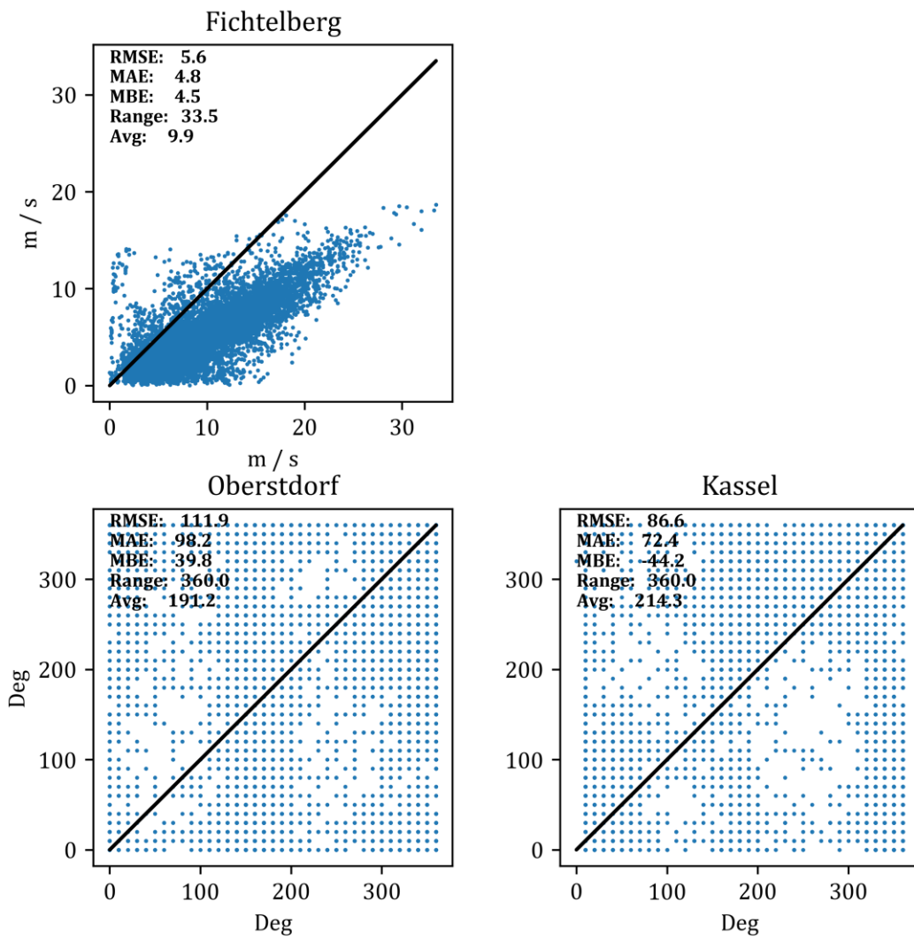
Figure 9: Worst fits of COSMO data and observation data for wind speed, which coincidentally are one of the worst direction results. On top wind speed and at the bottom the wind direction scatter plots. Fichtelberg has all, highest RMSE, MAE and |MBE|, and Oberstdorf has the highest RMSE and MAE, while Kassel has the highest |MBE| for wind direction.
