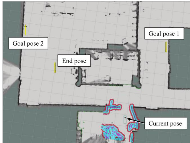
Fig. 3. Generated map of the environment with goal poses of the inspection mission.
