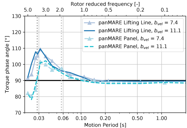
Figure 15. Phase shift between rotor torque and surge position corresponding to amplitudes of the model rotor shown in Fig. 12.
