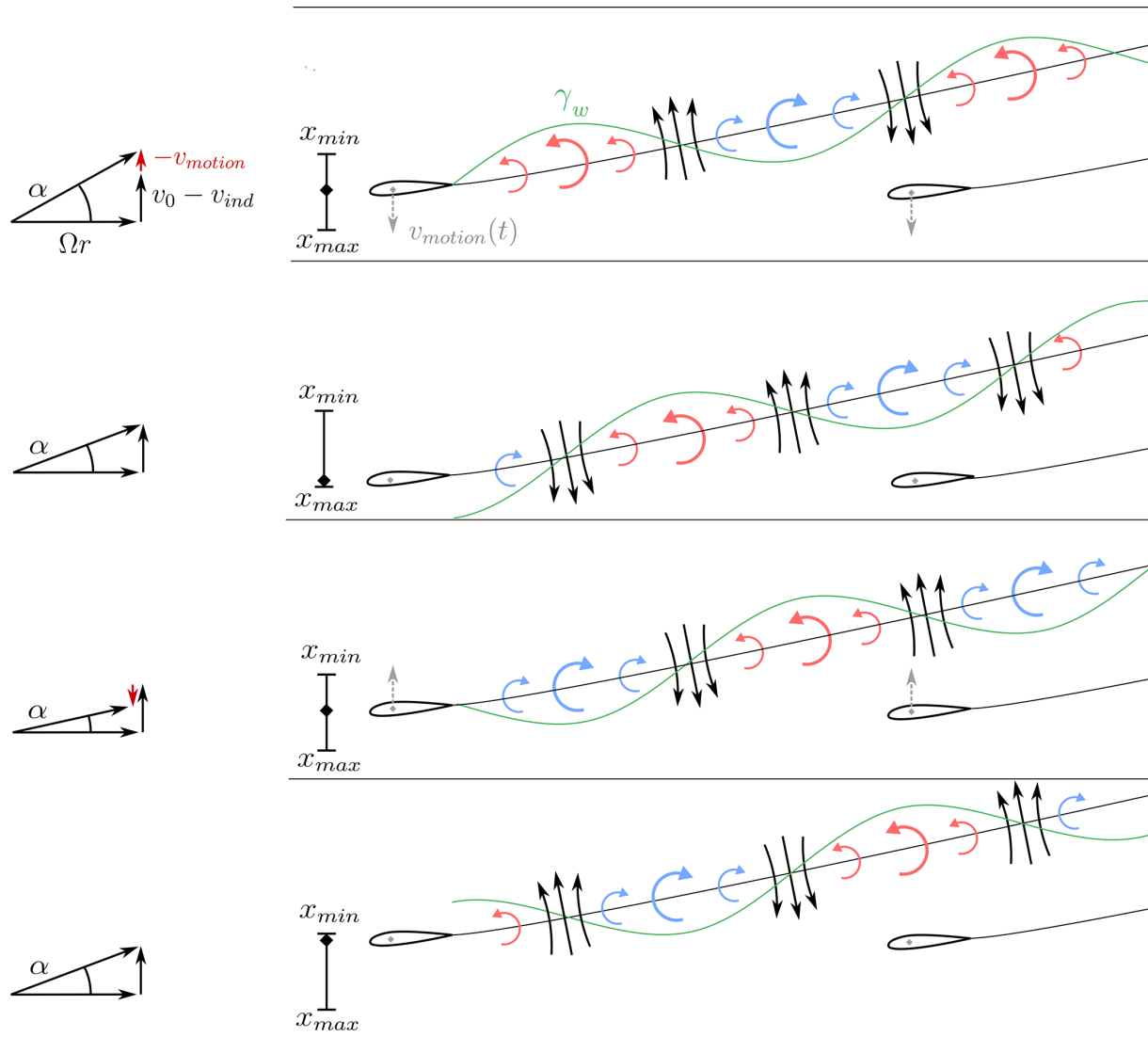
Figure 1. Schematic sketch of the vortex shedding at four steps during a surge motion cycle in the two-dimensional projection. The actual surge motion position varies between x_{\min} (turbine moved in wind direction) and x_{\max} (turbine moved against wind direction). Dashed grey arrows illustrate the motion velocity. Solid black arrows indicate the local flow direction. The green line represents the strength of the shed vorticity \gamma_w , which varies in a sinusoidal manner. The velocity triangle on the left gives an indication of the change in the angle of attack \alpha due to the variation in the motion velocity.
