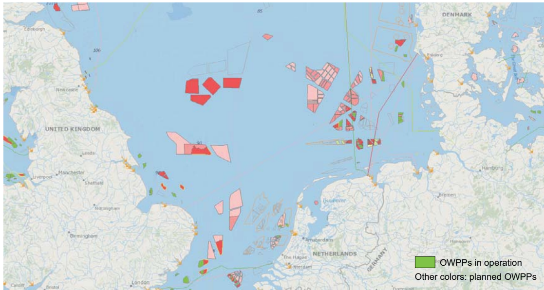
Figure 2.18: Operated and planned European OWPPs in the North Sea (4coffshore 2015a)
