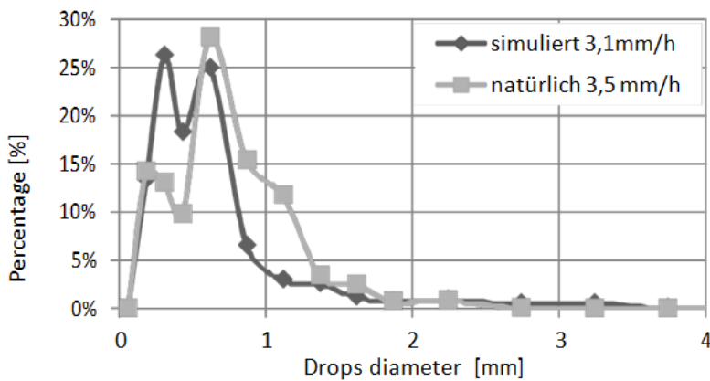
Figure 11. Comparison of drop diameters for natural and simulated (K60/M80) rain at an intensity of 3 mm/h
