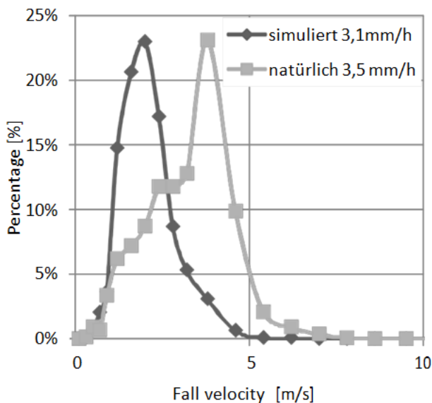
Figure 12. Comparison of fall velocities for natural and simulated rain at small intensities
