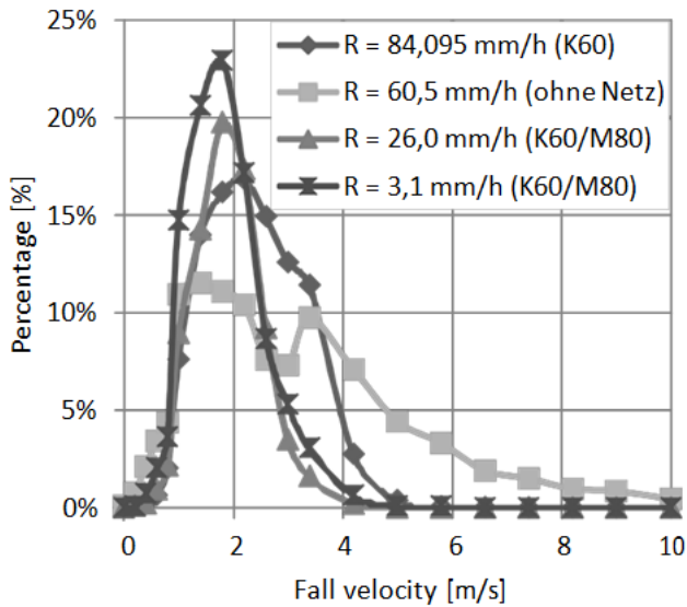
Figure 13. Comparison of fall velocities for different intensities
