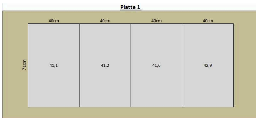
Figure 7. Spatial rainfall distribution on plate 1, measured with rainfall collectors
