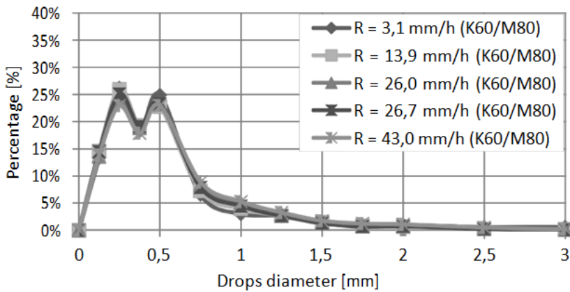
Figure 10. Drop size distribution for different intensities with net configuration (K60/M80)
