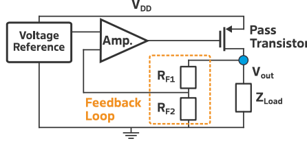
Fig. 15. Schematic of a generic low drop-out voltage regulator. Refer to [19] for background.
