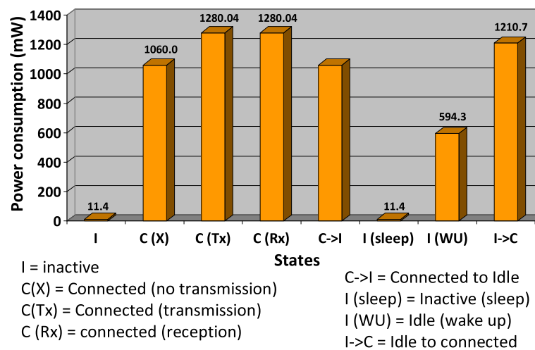
Fig. 15 A comparison of power consumption for different device states [144]
