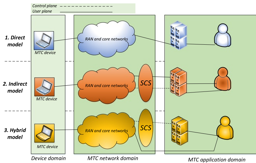
Fig. 11 3GPP direct, indirect, and hybrid models for MTC communications
