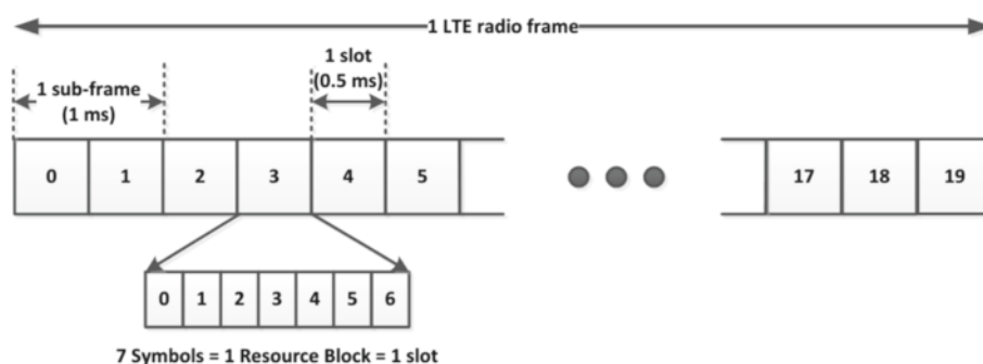
Fig. 6 LTE FDD frame structure [13]
