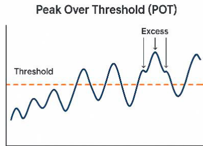
Fig 1: Illustration of the POT method. Data above the threshold (dashed line) are extracted as excess values for modelling the tail behaviour.
