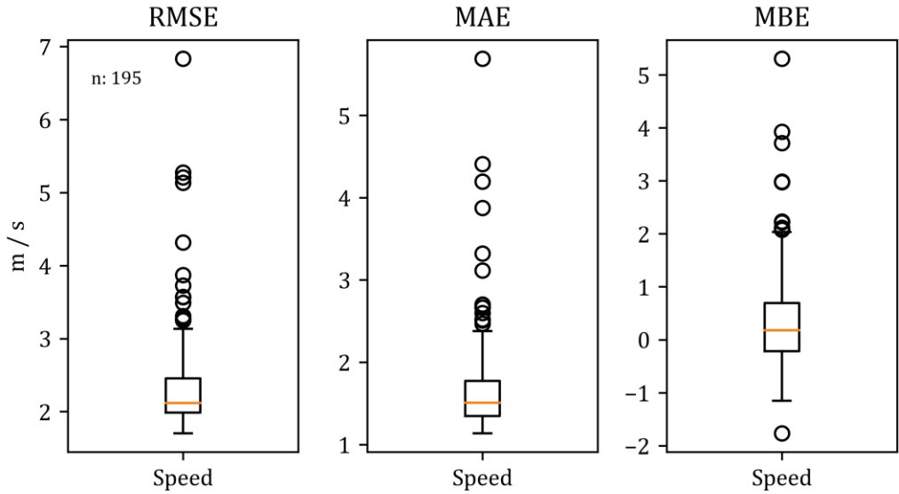
Figure 13: Overall statistical results for wind speed. Speed differences were accounted and are given in m/s. Size of dataset was n = 195.
