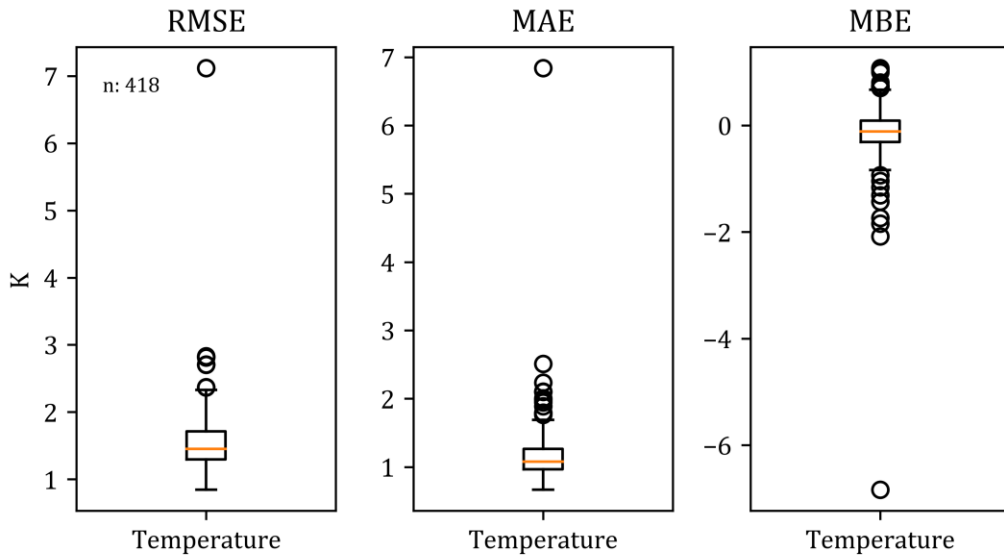
Figure 4: Overall statistical results for temperature. Temperature differences were accounted and are given in Kelvin. Size of dataset was n = 418.
