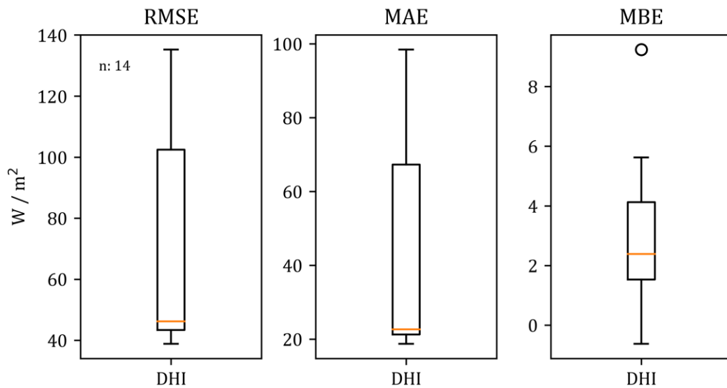
Figure 7: Overall statistical results for diffuse irradiation (ASWDIFD/DHI). Irradiation differences were accounted and are given in W/m^2 . Size of dataset was n = 14 .
