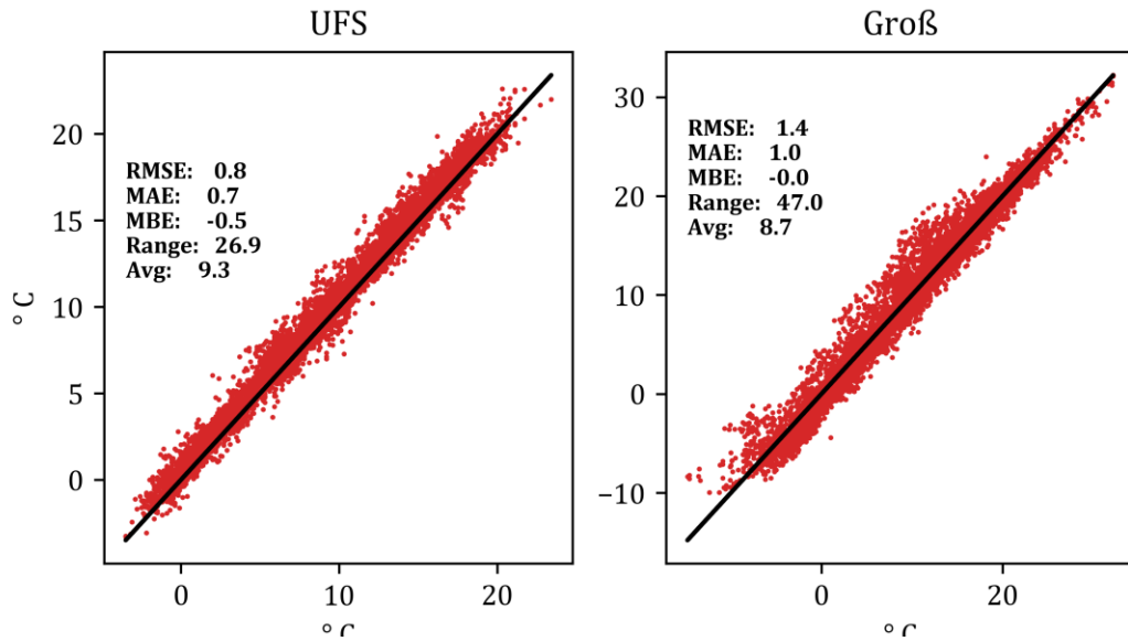
Figure 6: Best fits of COSMO data and observation data. The best in RMSE and MAE is UFS and in |MBE| Groß.
