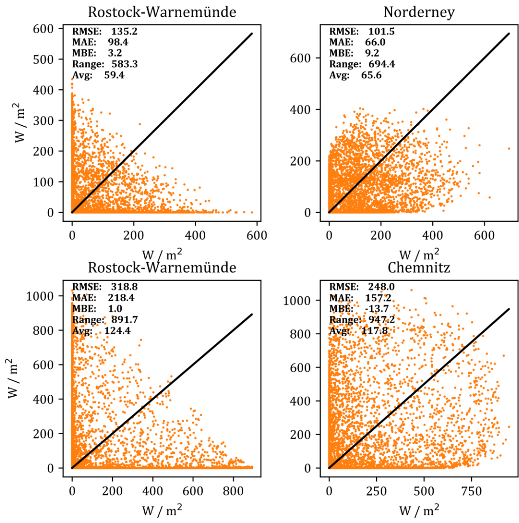
Figure 9: Worst fits of COSMO data and observation data. On top the diffuse irradiation and at the bottom the global irradiation scatter plots. Rostock-Warnemünde has both highest RMSE and MAE for DHI and for GHI. Norderney and Chemnitz have highest |MBE| in DHI and GHI respectively.
