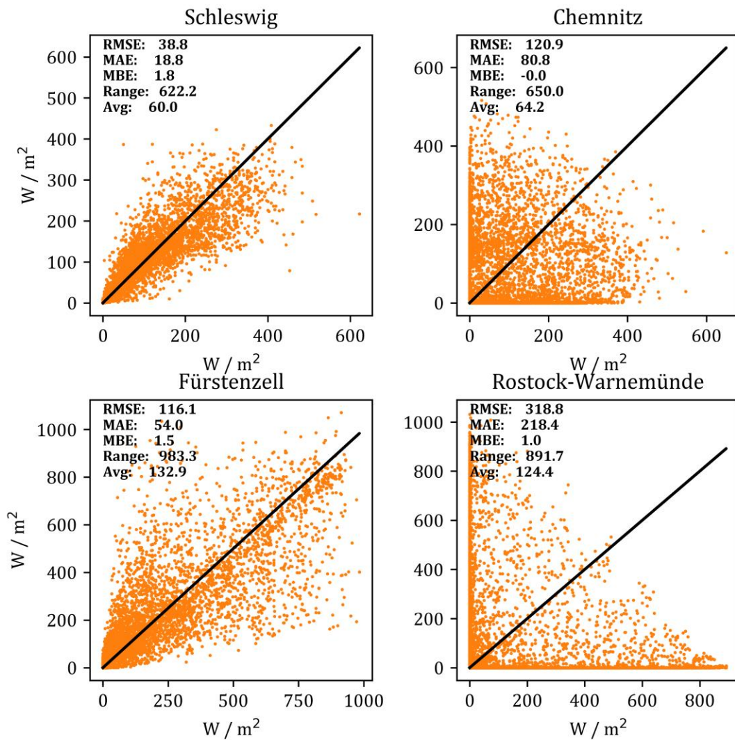
Figure 10: Best fits of COSMO data and observation data. On top the diffuse irradiation and at the bottom the global irradiation scatter plots. Schleswig has both lowest RMSE and MAE in DHI, while Fürstenczell has both lowest RMSE and MAE for GHI. Chemnitz and Rostock-Warnemünde both have the lowest |MBE|.
