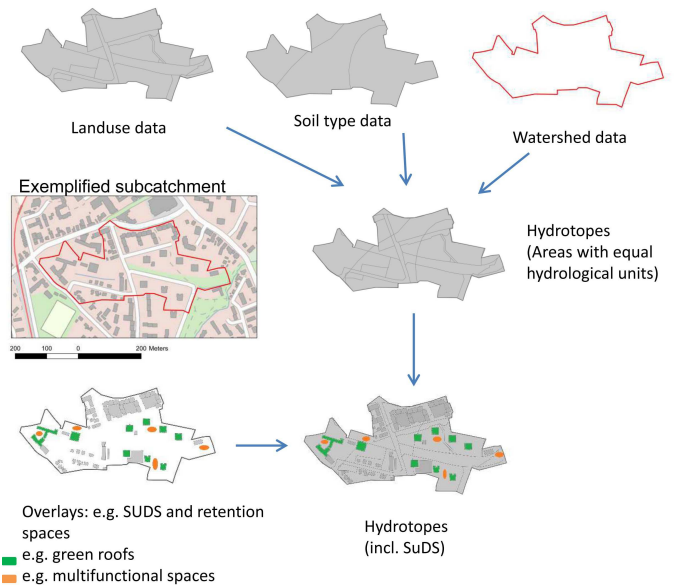
Figure 1 Spatial mapping (intersection and aggregation) to define equal hydrological response units containing the SUDS information as additional attributes (adopted from (Hellmers et al. 2016)).
