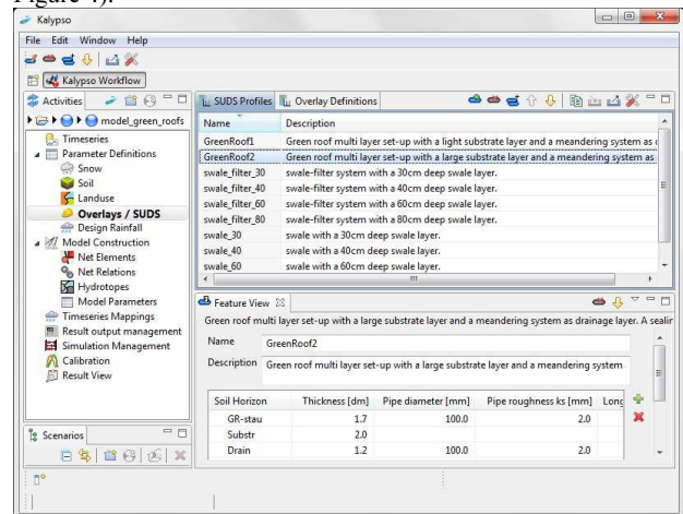
Figure 4 Workflow of KalypsoHydrology and parameter set-up for multiple layer elements (e.g. SUDS)
