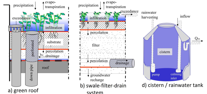
Figure 2 Schematic design of SUDS (from left to right): green roof, swale-filter-drain system, cistern (adopted from (Hellmers et al. 2016)).
