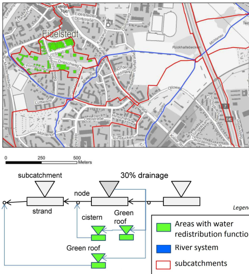
Figure 3 Implementation of overlays (here: green roofs and cisterns) in the system plan of a semi-distributed RRM (adopted from (Hellmers et al. 2016))
