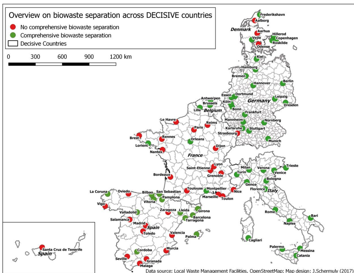
FIGURE 4: Overview on biowaste separation of exemplarily selected (not all) cities of the six DECISIVE countries Belgium, Denmark, France, Germany, Italy and Spain.
