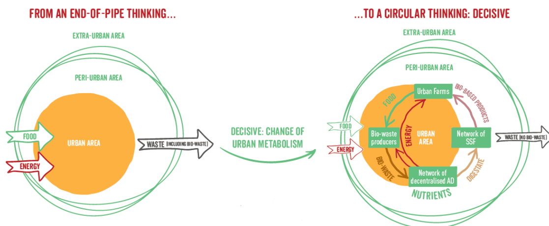
FIGURE 1: DECISIVE vision towards a decentralised biowaste management.
