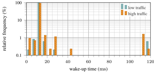
Fig. 2. Distribution of wake-up intervals for beacon reception vs. background traffic of ten 5 s time windows with a beacon interval of 102.4 ms.
