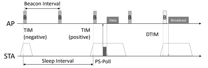
Fig. 1. Sleep Intervals in PSM
