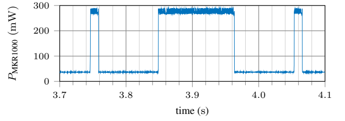
Fig. 4. Missing one beacon leads to a whole period spent in receive mode.
