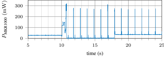
Fig. 3. Wrong implemented standby mode of Arduino in standard library.
