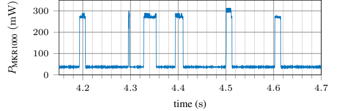
Fig. 5. Strongly varying reception times in power save mode.
